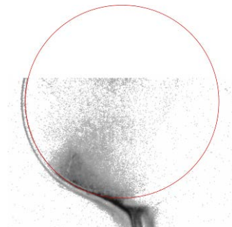
Figure 4: Light-sheet picture of the rhodamine concentration in the center plane of the sphere. A red circle indicates the contour of the sphere and next to it the boundary layer (thickness is about \delta/D = 0.023 ).
