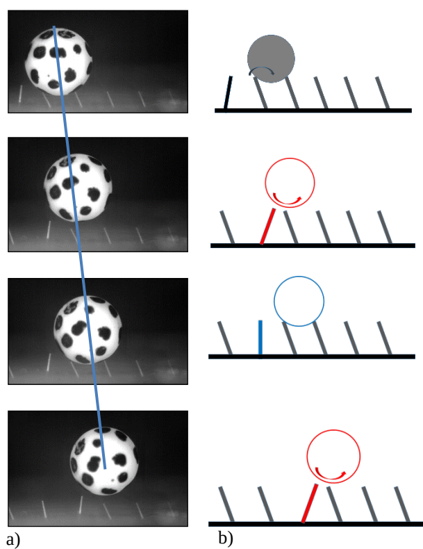
Figure 5. Symplectic transport of a sphere along the ciliated wall. Pulse propagation is from left to right at a speed of 12 \Delta s/\text{sec} ( 12 \text{ mm}/\text{sec} ). Mean particle speed in transport direction U_p=U is equal to wave propagation speed. Spin of the particle is counter-clockwise. Number of active flaps in a pulse is one.
