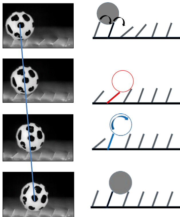
Figure 6. Antiplectic transport of a sphere along the ciliated wall. Pulse propagation is from right to left at a speed of 12 \Delta s/\text{sec} ( 12 \text{ mm/sec} ). Mean particle speed in transport direction is U_p = \Delta s/T which is one flap per wave cycle. Spin of the particle is clockwise. Number of active flaps in a pulse is two.
