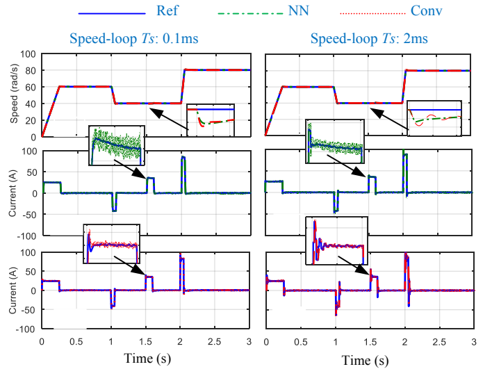
Fig. 11. NN vs. conventional - Load disturbance and speed-loop sampling time impacts: (a1)&(b1) reference/actual motor rotational speeds, (a2)&(b2) reference/actual d -axis currents using NN control, (a3)&(b3) reference/actual q -axis currents using conventional PI control
