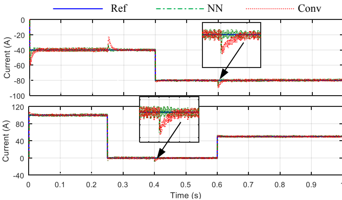
Fig. 10. NN vs. conventional for 40% increase of rotor flux linkage
