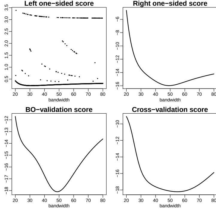
Figure 1: Mortality data: bandwidth selection scores with multiplicative bias corrected hazard estimator.
