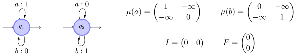
■ Figure 1 Graph and matrix representations of a max-plus automaton.
