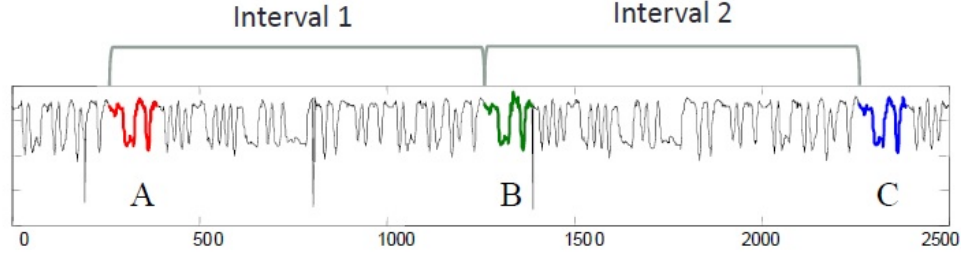
Figure 7: A motif or recurring pattern which repeats three times, in positions A, B and C, in test data. Source: Eamonn Keogh (reproduced with permission).
