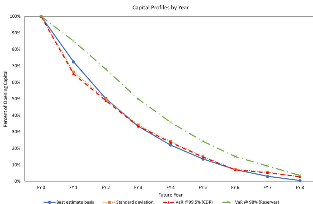
Figure 1: Capital profiles associated with Table 9, including VaR at 98% of the discounted outstanding reserves in each future year (see Section 6).
