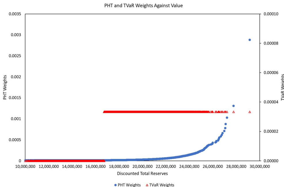
Figure 2: TVaR and PHT weights against simulated total discounted reserves.
