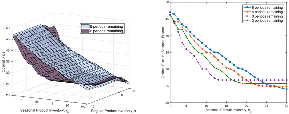
(a) Optimal Price for (i) 2 periods and (ii) 5 periods (b) Optimal Price for x_r = 0 and across various periods remaining in the selling horizon
