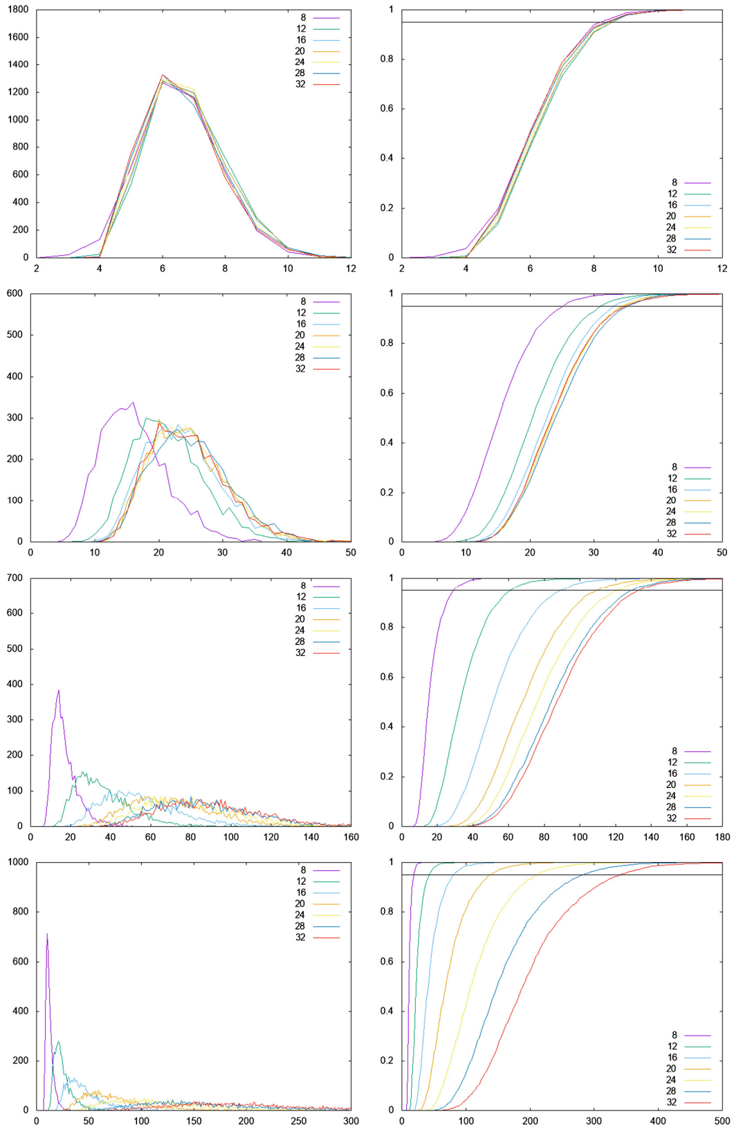
Fig. 11. Frequency and cumulative distributions for 2-, 4-, 8- and 16-dimensional completion.
