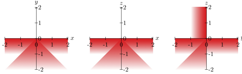
Fig. 2. \pi_{\{x,y\}}(C') , \pi_{\{x,z\}}(C') and \pi_{\{y,z\}}(C') .
