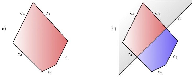
Fig. 9. Insertion and filtering.
