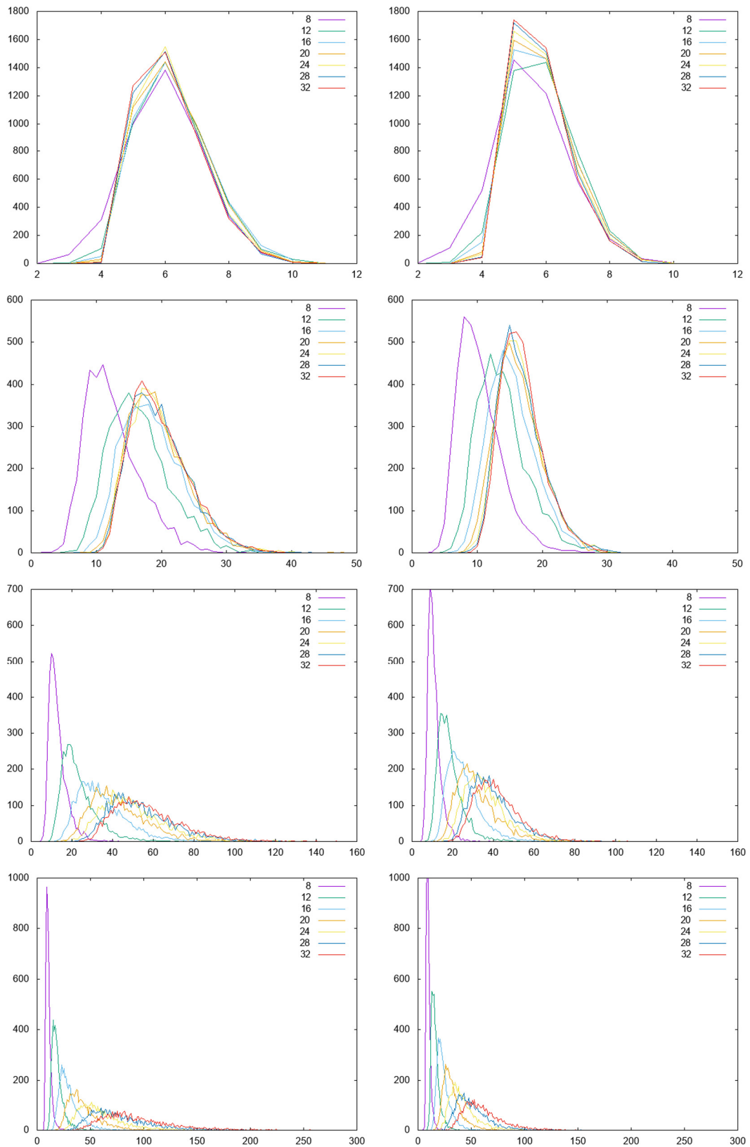
Fig. 12. Frequency distributions for Logahedra (left) and Octagons (right).
