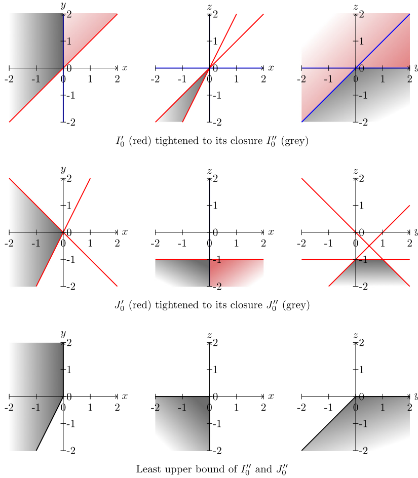
Fig. 1. Closure and least upper bound. (For interpretation of the colours in the figure(s), the reader is referred to the web version of this article.)
