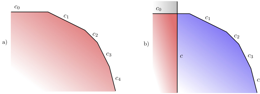
Fig. 10. Insertion and filtering for an unbounded two variable projection.
