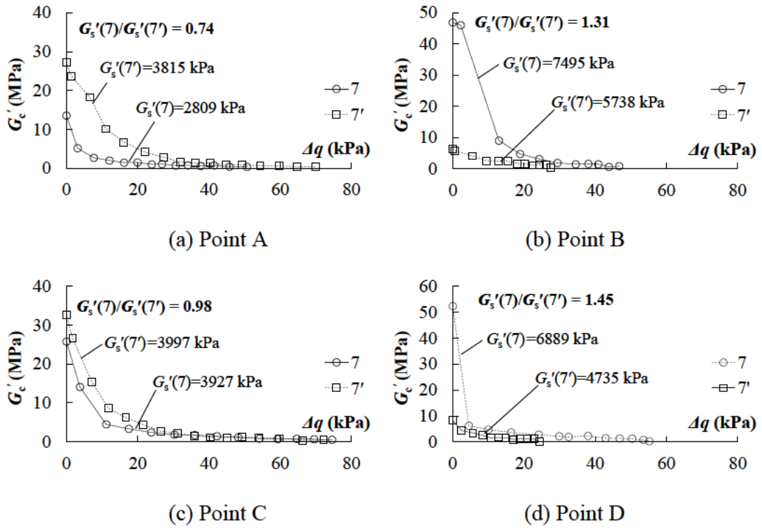
395 Fig. 12 Comparison of soil stiffness during step 7 in both case 1 and case 2
