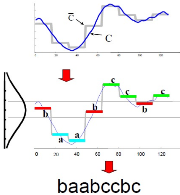
Figure 2: Symbolic Aggregate Approximation (SAX). An original real-valued time series C (top) is discretized using the Piecewise Aggregate Approximation (PAA) algorithm resulting in \bar{C} . The discrete values are assigned a symbol such that every symbol is equally likely to occur according to the standard Normal distribution. C is converted to a symbol string baabccbc . Source: Eamonn Keogh (reproduced with permission).
