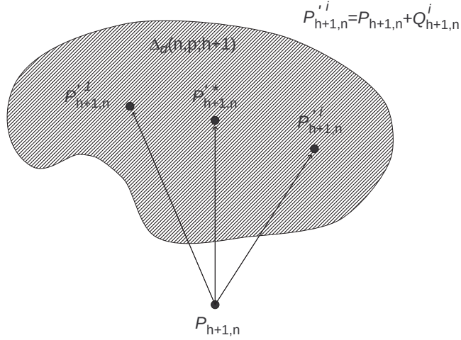
Figure 1: The notion of “approximate GCD”
