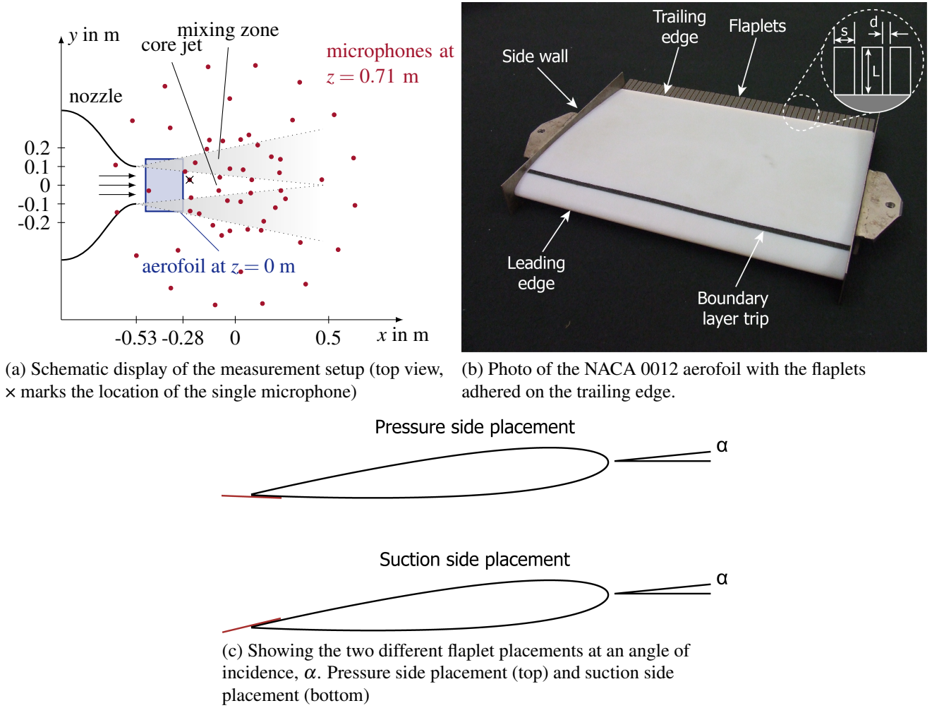
Figure 1: Experimental set-up
