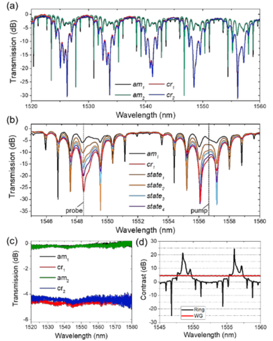
Fig. 4. (a) Measured transmission spectra of the ring resonator device over two phase-change cycles. (b) Intermediate transmission spectra when the GST is partially crystallized. (c) Measured transmission spectra of a GST-loaded straight waveguide over two phase-change cycles. (d) Transmission contrast between the crystalline and amorphous states.
