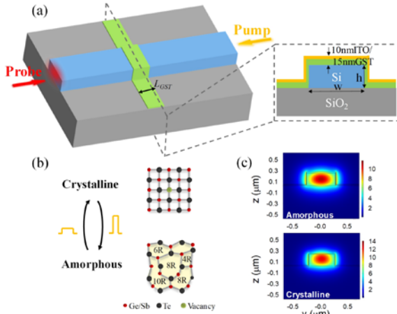
Fig. 1. (a) Schematic structure of the GST-loaded silicon waveguide. The inset shows the cross-sectional view of the Si-GST hybrid waveguide section. (b) Reversible phase change of GST material. (c) Simulated modal electric-field profiles of the Si-GST hybrid waveguide for the two phase states.
