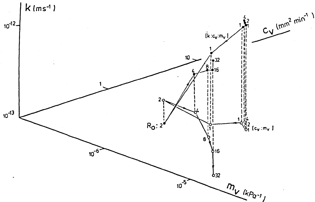
Figure 8.40 k : c_v : m_v relationship, till W(d) . (Reconstituted)
