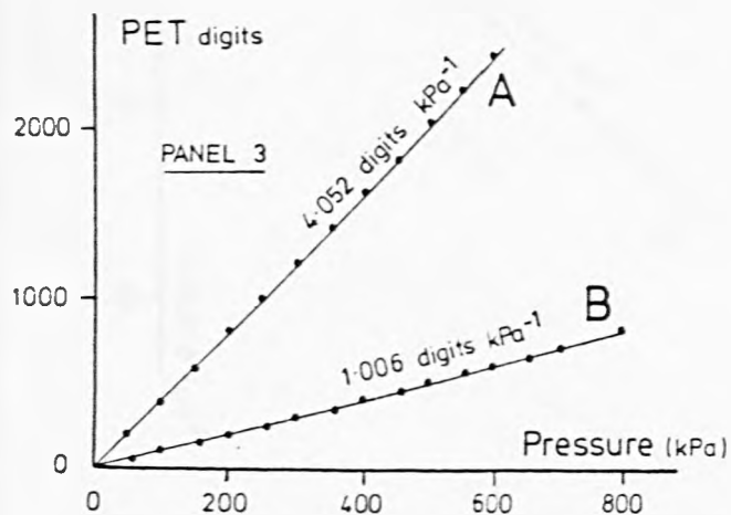
Figure 6.8 Pore pressure transducer calibration graphs , panels 1 - 4 .
