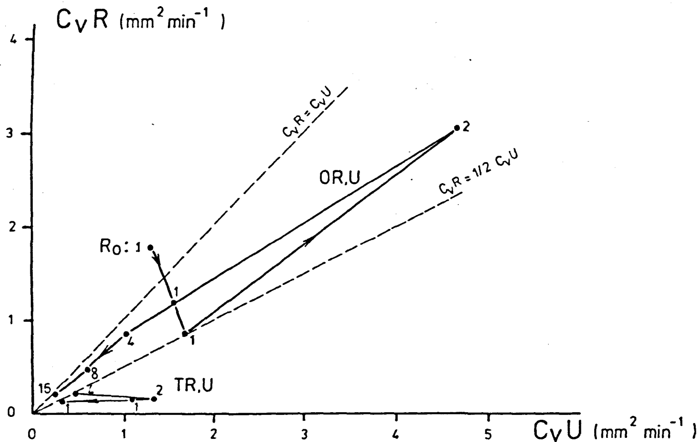
Figure 8.25 \frac{C_V R}{C_V U} : \frac{C_V U}{C_V U} : \text{till HH(a)} (Tests OR(1) , OU(1)U ; TR(1) , TU(1) ).
