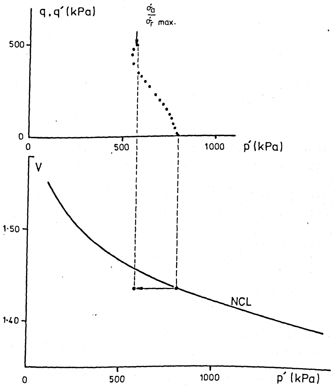
Figure 7.43 q, q' : p' and V : p' : RA1(11).
