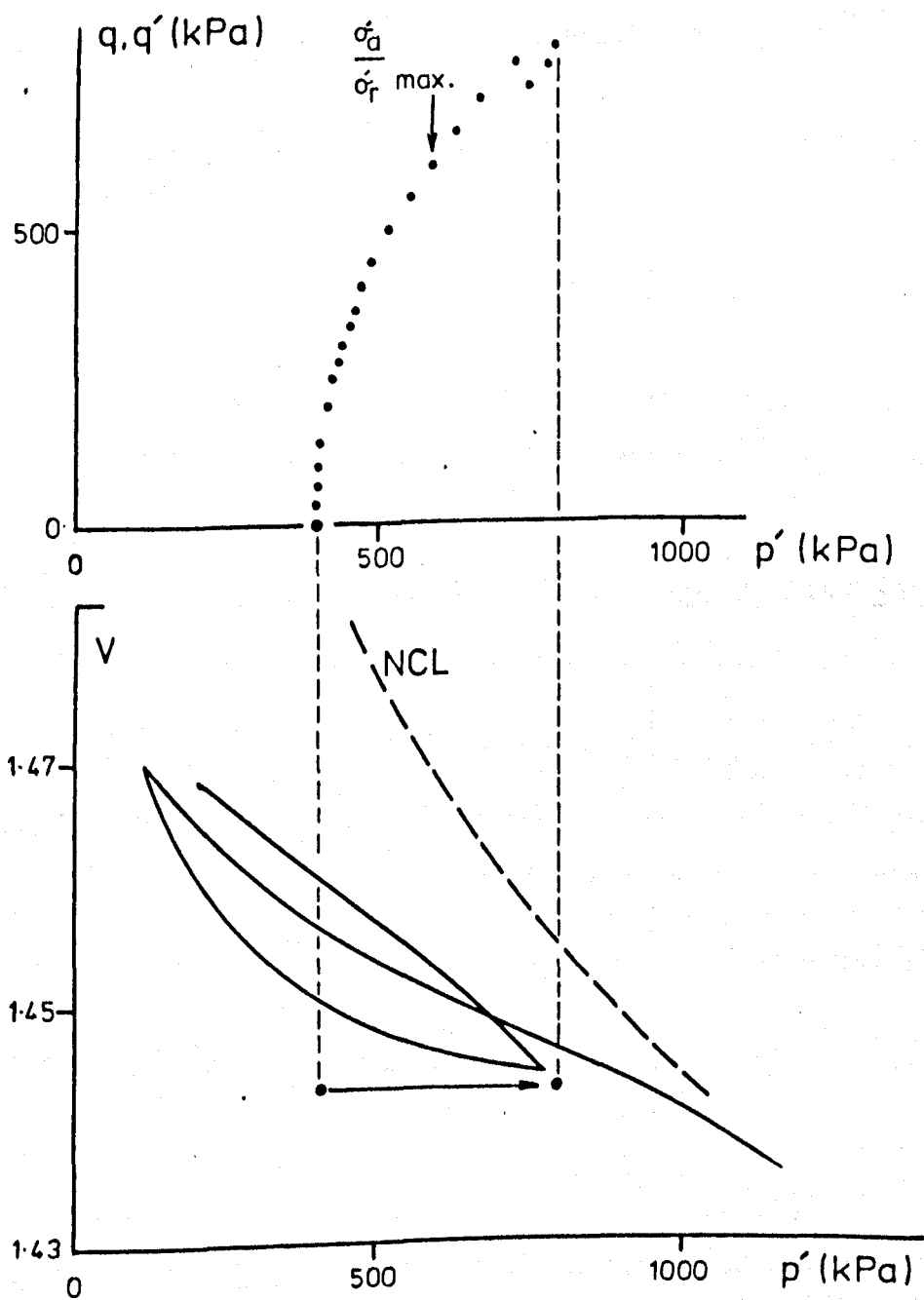
Figure 7.58 q, q' : p' and V : p' : UA2(111).
