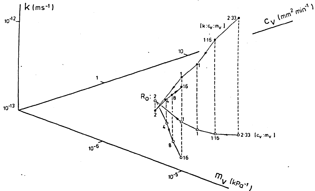
Figure 8.39 \underline{k : c_v : m_v} relationship, till W(b) , (Undisturbed)
