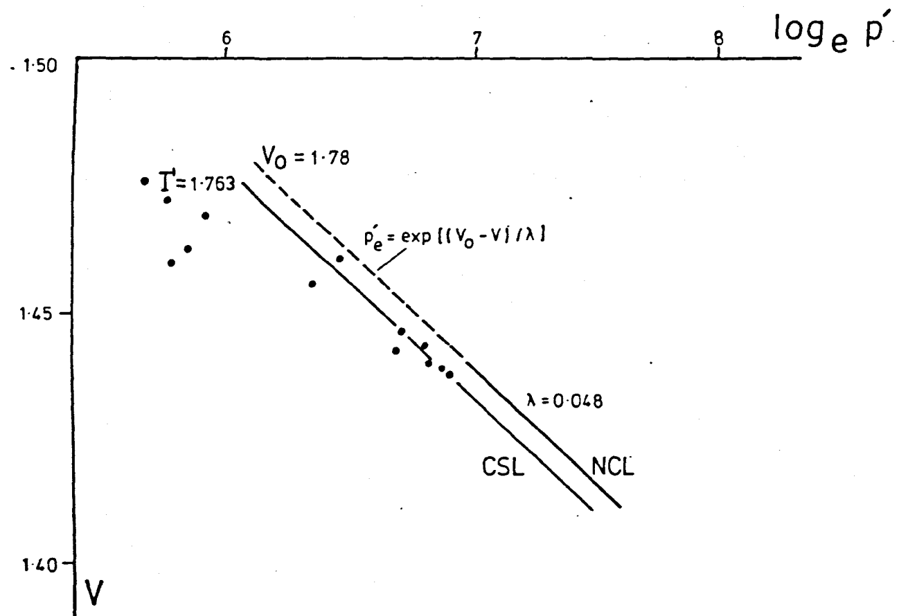
Figure 8.48 \log_e p' : V , undisturbed till HH(a).
