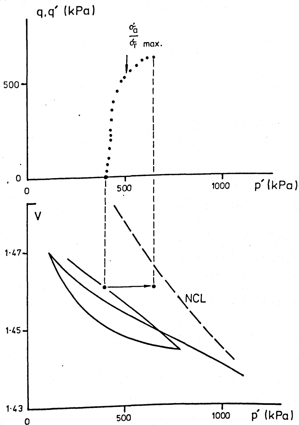
Figure 7.52 q, q' : p' and V : p' : \text{UA1(1)} .
