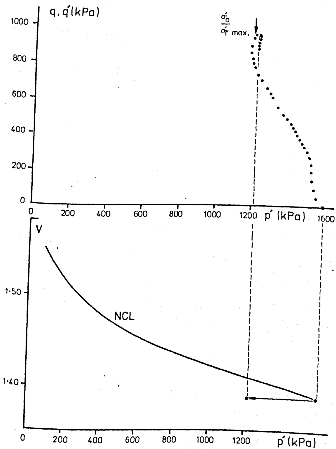
Figure 7.44 q, q' : p' and V : p' : \text{RA1(111)} .
