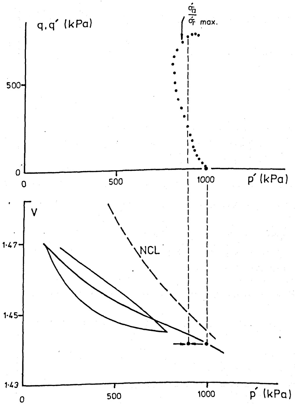
Figure 7.54 q, q' : p' and V : p' : \text{UA1(III)} .
