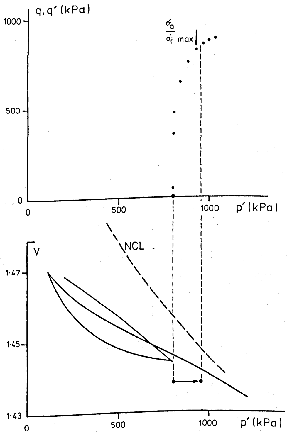
Figure 7.59 q, q' : p' and V : p' : UB(1) .
