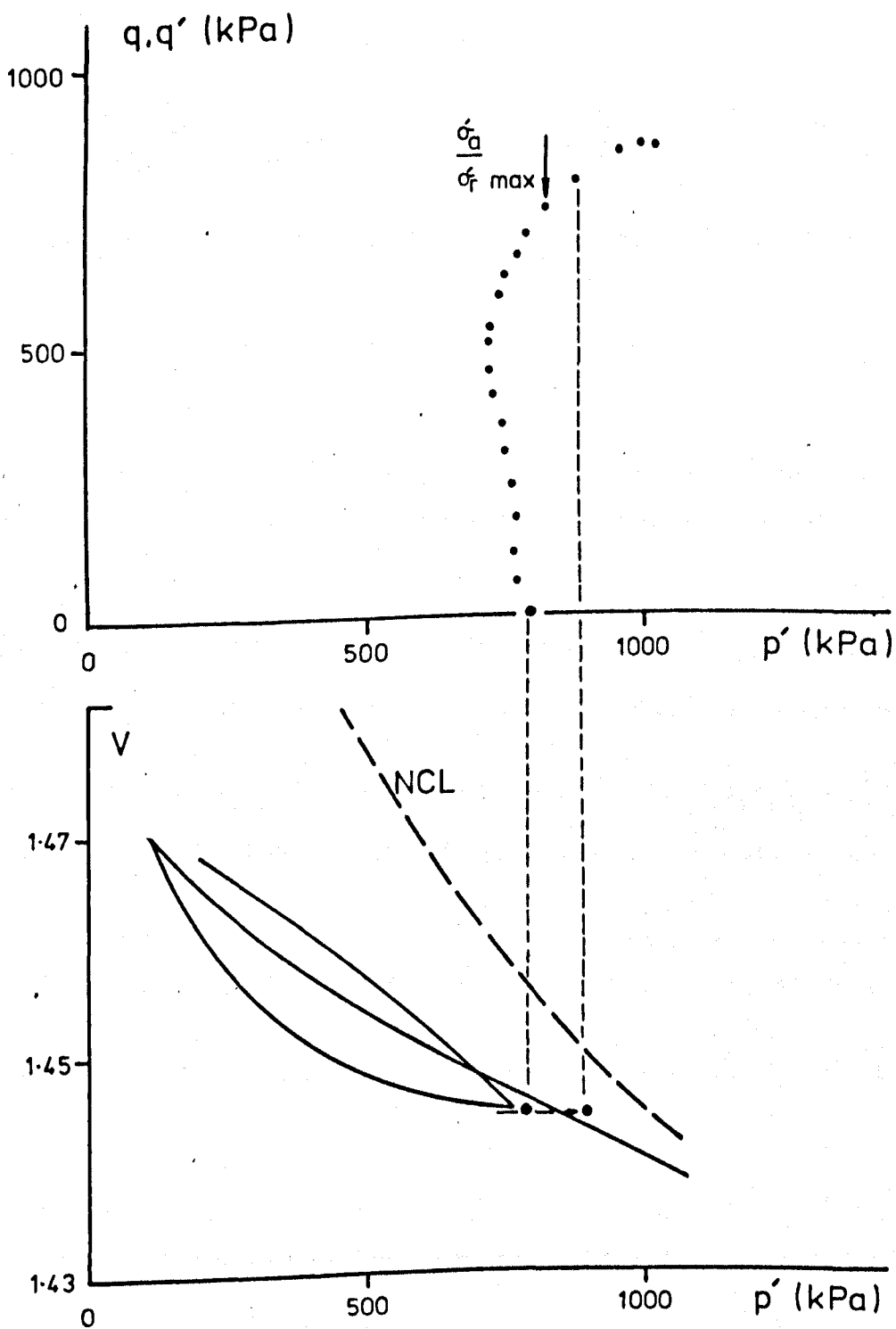
Figure 7.53 q, q' : p' and V : p' : UA1(11).
