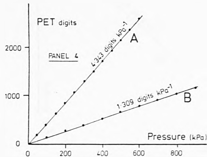
Figure 6.8 Pore pressure transducer calibration graphs , panels 1 - 4 .
