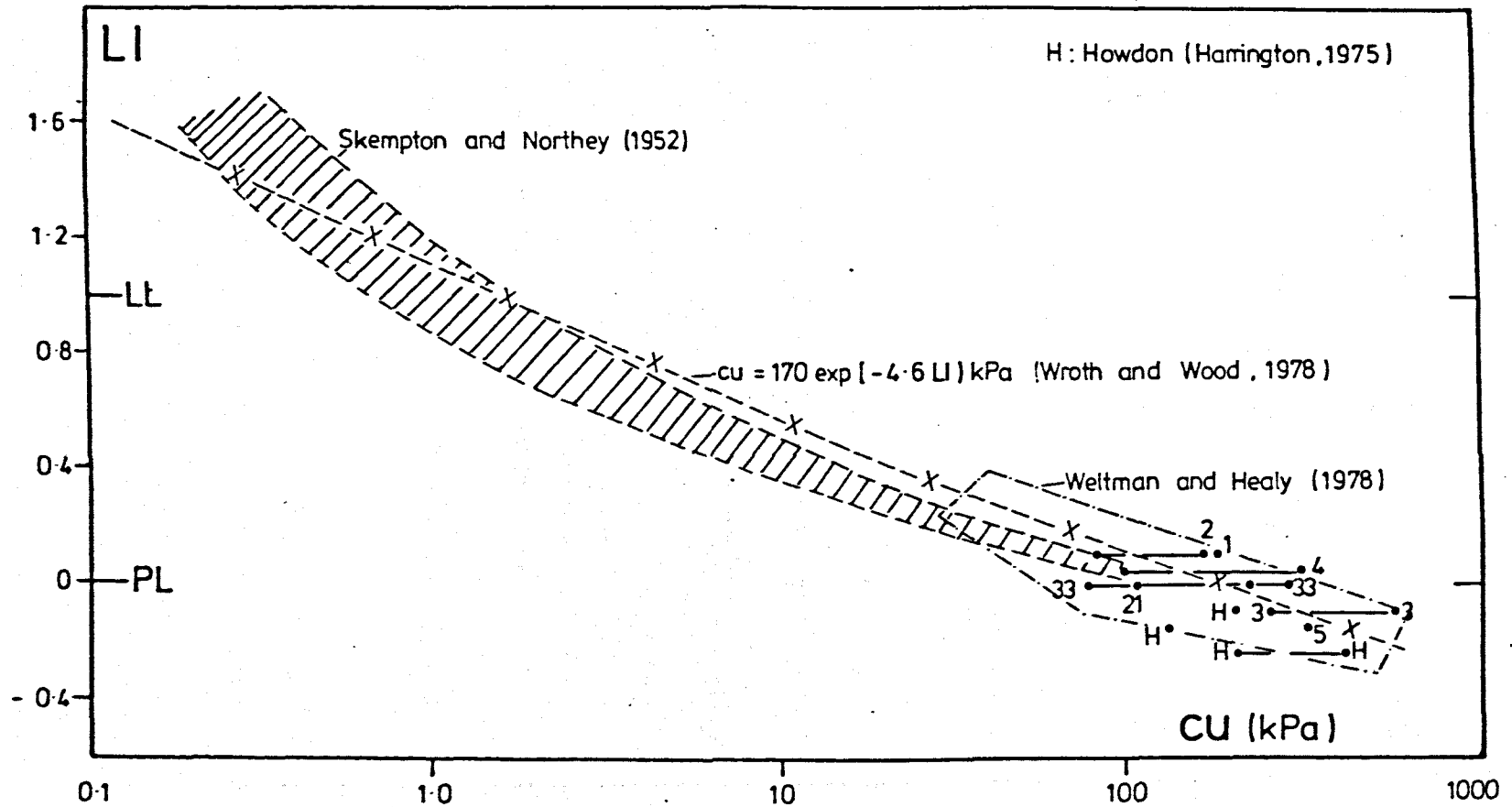
Figure 4.10 Relationship between undrained shear strength and liquidity index for U.K. tills.
