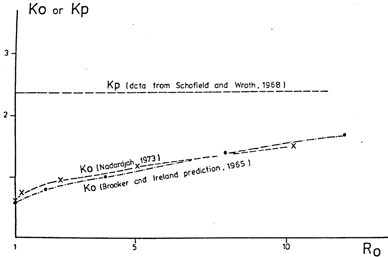
Figure 8.2 Variation of K_o with overconsolidation ratio for one-dimensionally unloaded kaolin.
