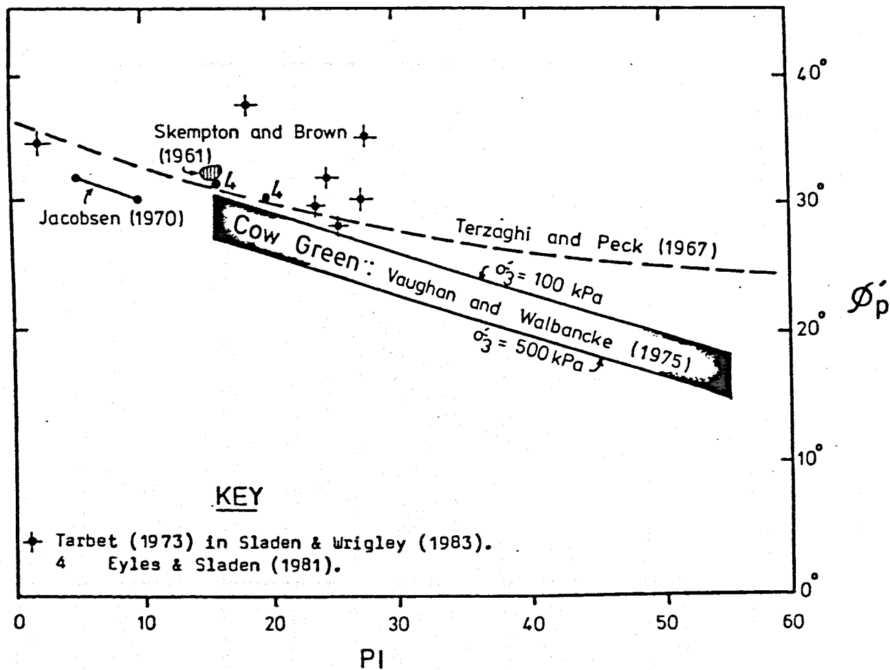
Figure 4.12 \phi_p' : PI for various lodgement tills. (Based on Sladen and Wrigley, 1983).
