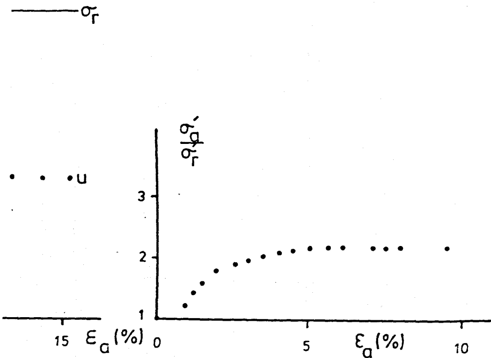
Figure 7.31 CU triaxial test results : UA1(v).
