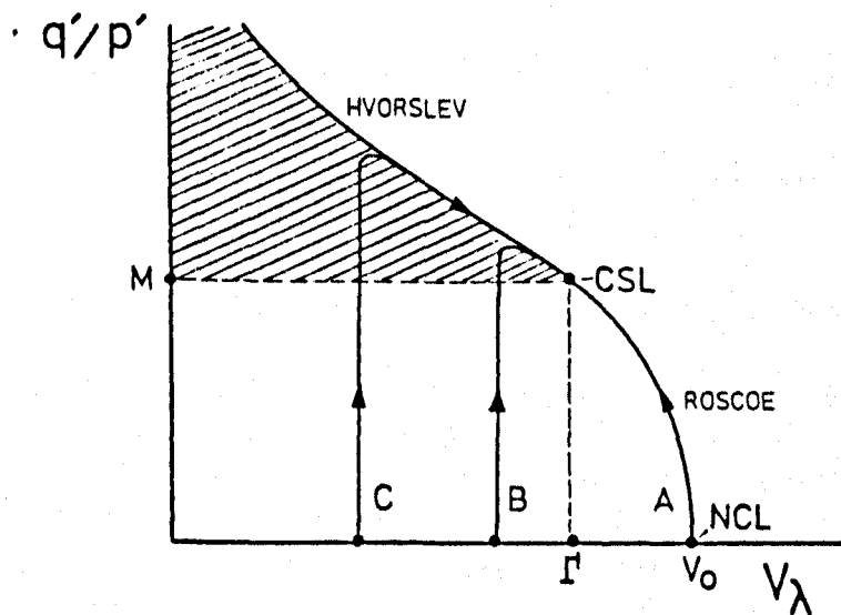
Figure 3.5 The reference section in q'/p' : V_\lambda space.
