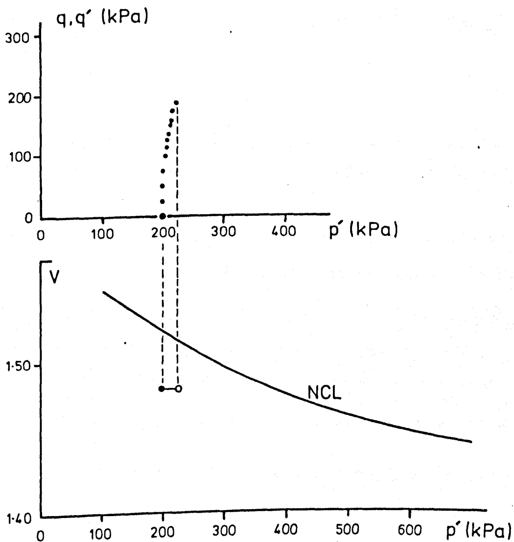
Figure 7.48 q, q' : p' and V : p' : RB(111).
