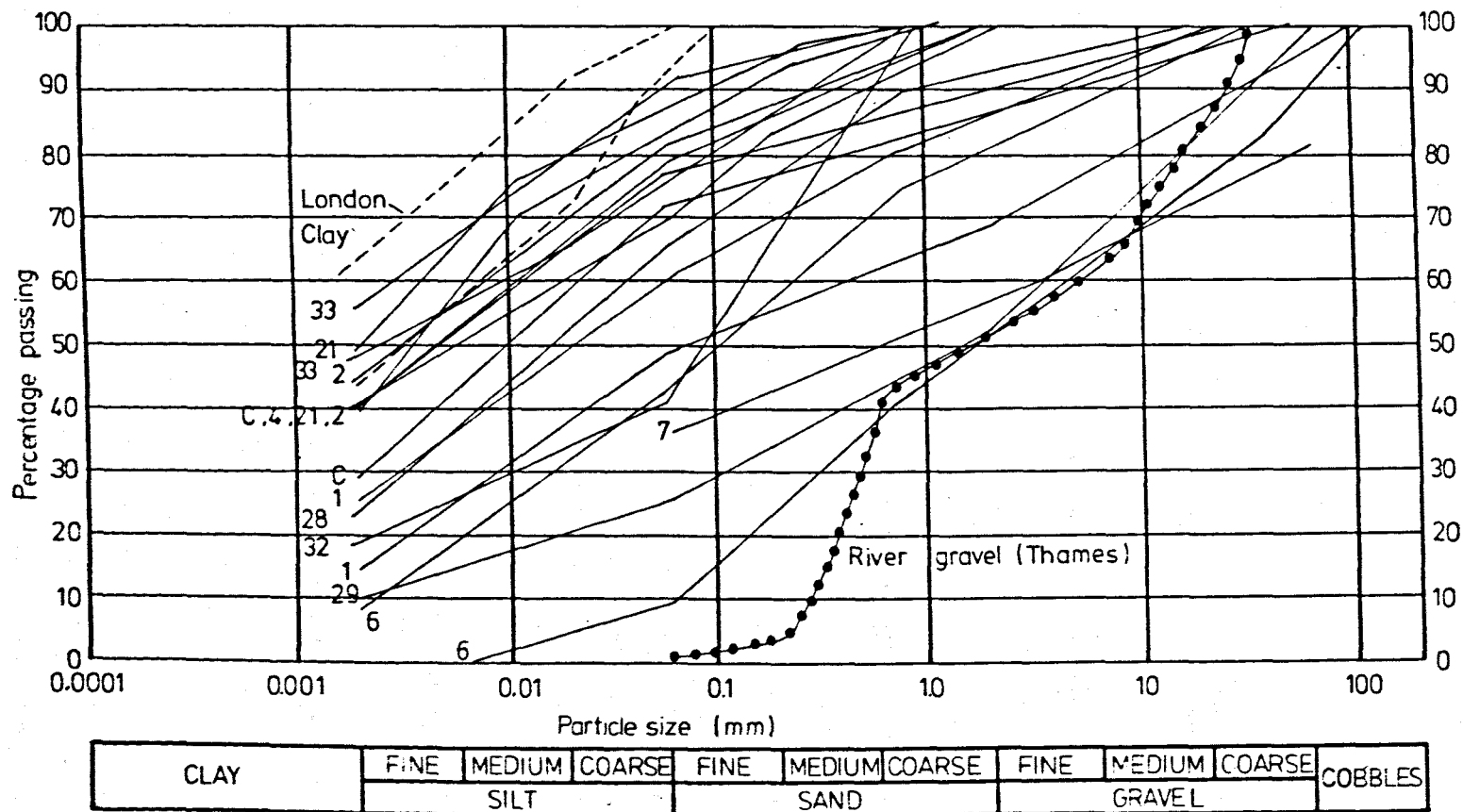
Figure 4.3 Grading characteristics of lodgement tills in the U.K. (Key as in Table 4.2 : C = Cowden Till, Powell et al, 1983).
