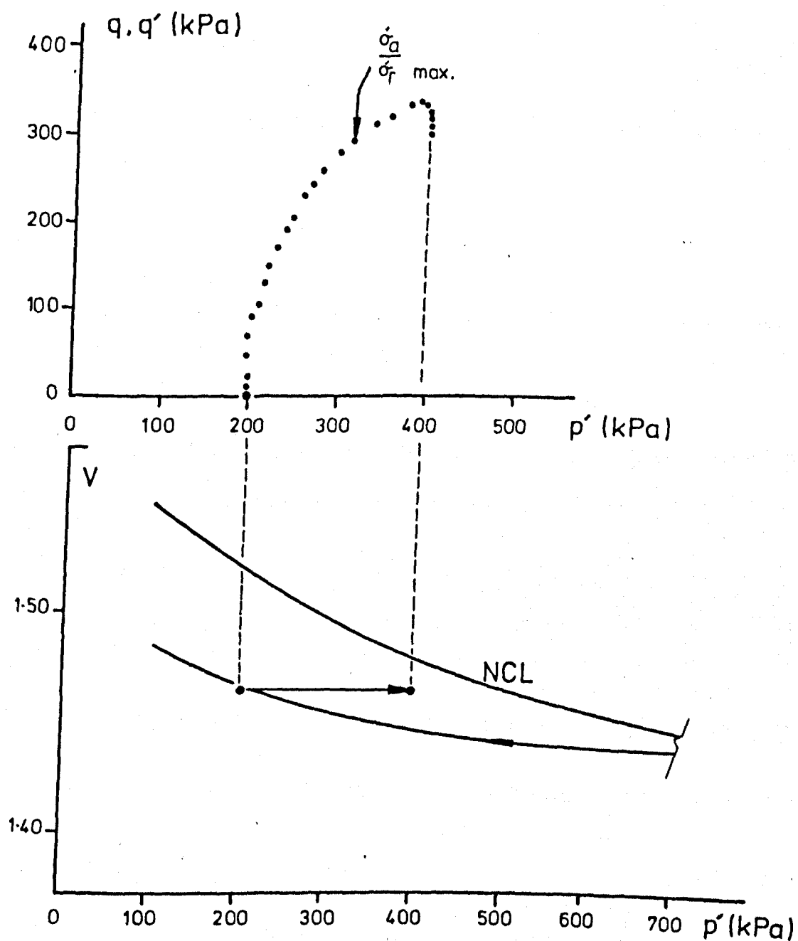
Figure 7.45 q, q' : p' and V : p' : RA2(11) .
