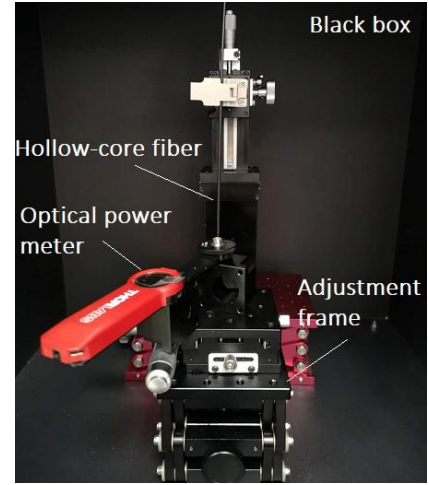
Fig. 5. Fiber optic probe measurement adjustment frame showing the key components of the measurement system
