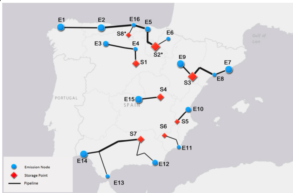
Figure 3. CO 2 pipeline and storage deployment in Spain
