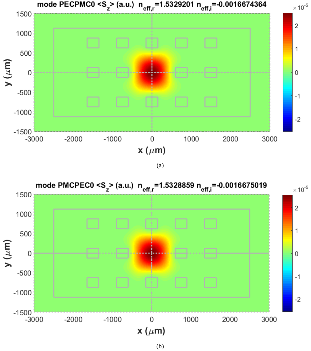
Fig. 12. The longitudinal component of time-averaged Poynting vector for modes of PCF-like structure using rectangular air holes within LDPE host (a) q-TE 00 , \alpha=3.033 dB/cm, and (b) q-TM 00 , \alpha=3.033 dB/cm.
