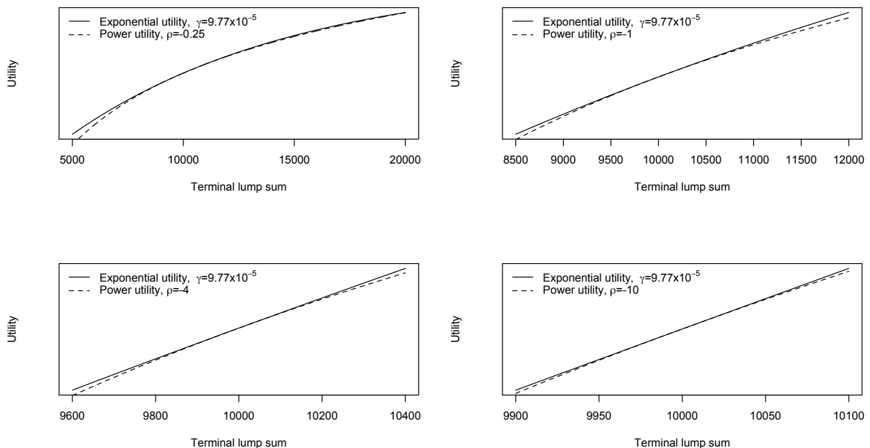
Figure 1: Comparison of the exponential utility (with parameter \gamma = 9.77 \times 10^{-5} yielding C = 9,480 ) against the power utility with varying parameter \rho = -0.25, -1, -4, -10 .
