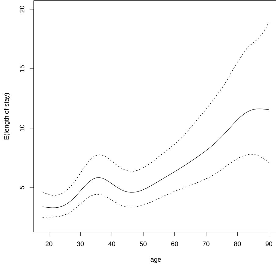
Figure 5: Effect of age on the the mean of hospital stays (black continuous line). The dashed lines represent 95% confidence intervals.
