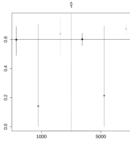
(b) Estimates for Kendall's \tau = 0.6 .
