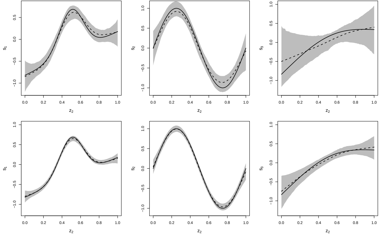
(b) Smooth curve estimates for s_1(\cdot) , s_2(\cdot) and s_3(\cdot) .
