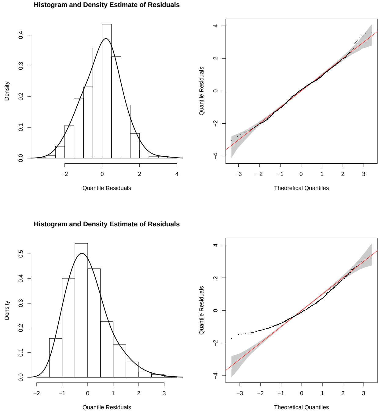
Figure 4: Histograms and Q-Q plots of normalized quantile residuals for length of hospital stay produced after fitting copula models based on the inverse Gaussian (top) and gamma (bottom) distributions. The QQ-plots also exhibit reference bands for judging the relevance of departures from the red reference lines. AIC and BIC values are 15413.15 and 16101.04 for the model with inverse Gaussian outcome distribution and 15616.74 and 16351.86 for the model with gamma distribution.
