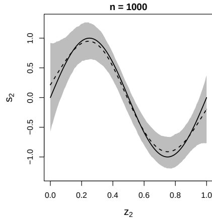
(a) Estimates for \beta_1 = -0.9 .
