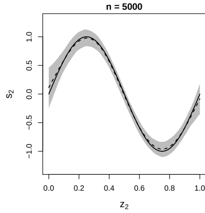
(b) Estimates for Kendall's \tau = 0.6 .
