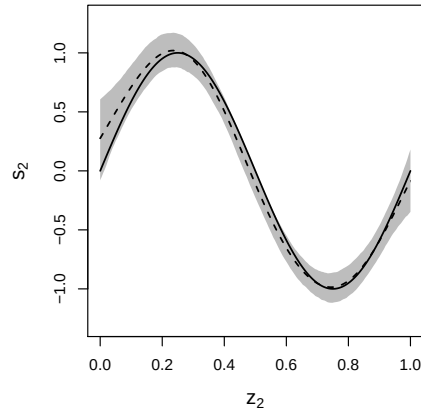
(c) Smooth curve estimates for s_2(\cdot) .
