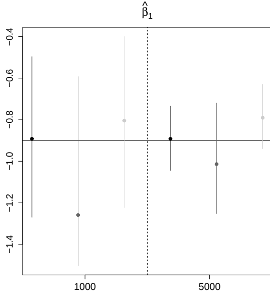
(a) Estimates for \beta_1 = -0.9 .
