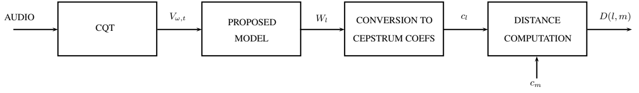
Figure 2: Diagram for the proposed acoustic scene classification system.
