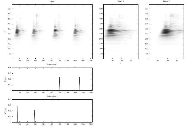
Figure 1: SIPLCA applied to a sequence of footsteps ( Z = 2 ). Top left: input constant- Q transform spectrogram, right: extracted time-frequency patches, bottom: extracted component activations.
