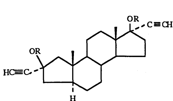
(4.2) , R = COEt (Anordrin)
