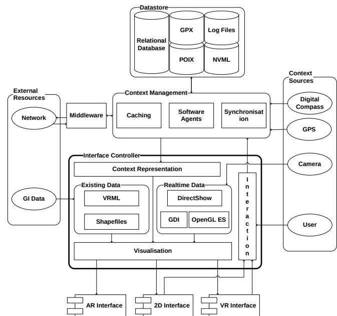
Fig. 1. Prototype Client Architecture
