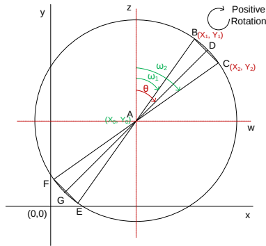
Fig. 4. Line & circle intersection for calculating the FOV
