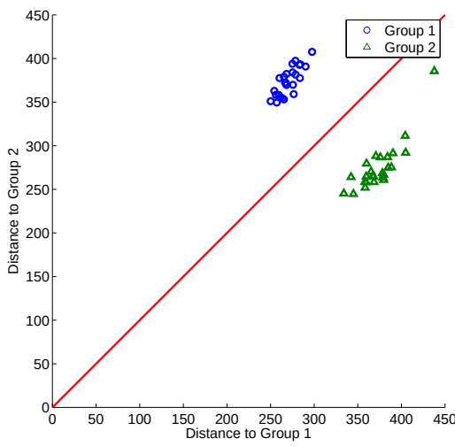
(c) SIMCA. p = 1250 , \frac{n_k}{p} = 0.02 .
