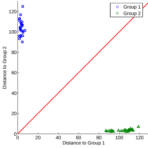
(a) SIMCA. p = 17 , \frac{n_k}{p} = 1.5 .
