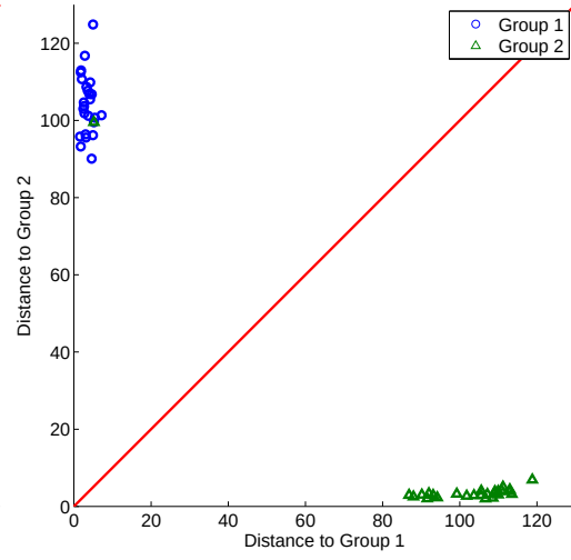
(b) SIMCA-D. p = 17 , \frac{n_k}{p} = 1.5 .
