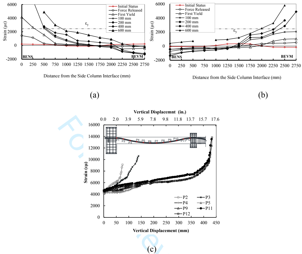
Fig. 16– Strain gauge results of PCSL-0.6: (a) top non-prestressed rebar; (b) bottom non-prestressed rebar; (c) prestressed tendon
