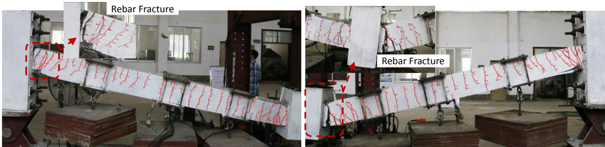
Fig. 10– Failure mode of PC specimen PCSH-0.6
