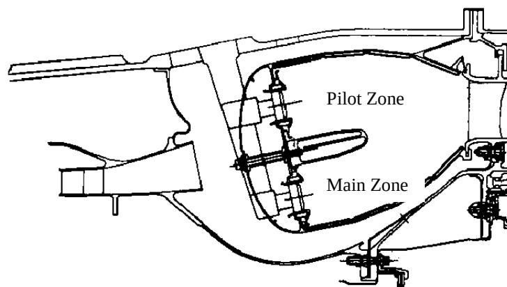
Figure 1. Side View of the Centre Section of the Double Annular Combustor
