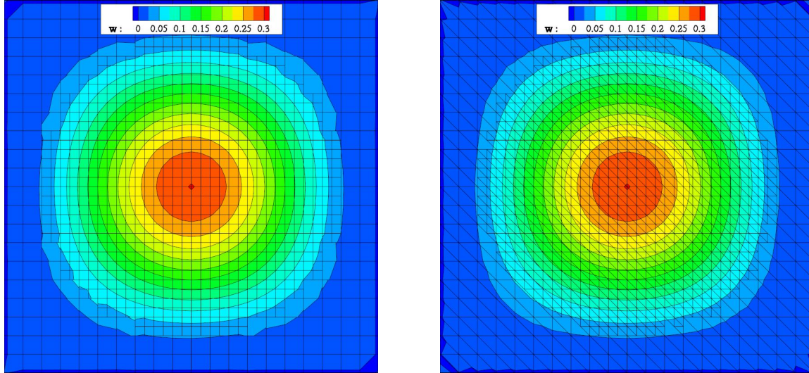
Figure 8: The final distribution of the w velocity for a square subdomain of the manufactured solution field with size L/2 Left: For a spatially refined unstructured hexahedral mesh. Right: For a spatially refined unstructured prismatic mesh.
