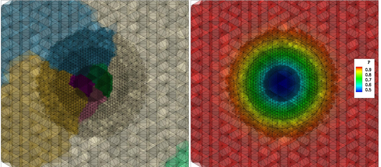
Figure 6: Left: Domain decomposition for a tetrahedral mesh refined to three levels. Different colours represent the mapping of different partitions. Right: Pressure distribution for an isentropic vortex projected on a tetrahedral grid.
