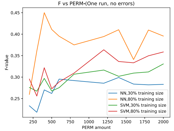
Fig. 6. Plot of permutation F -values up to PERM 2000.
