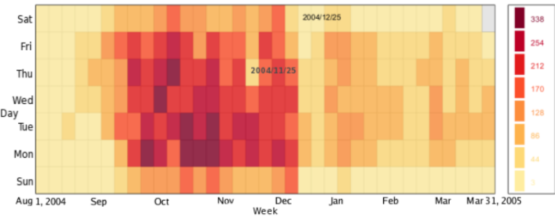
Fig. A.30 MobiVis (Shen and Kwan-Liu, 2008)
