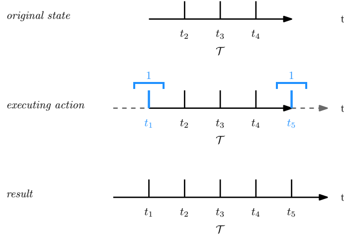
Fig. 6.19 Application of the Extend By operator, with durations 1 and 1 passed as parameters.
