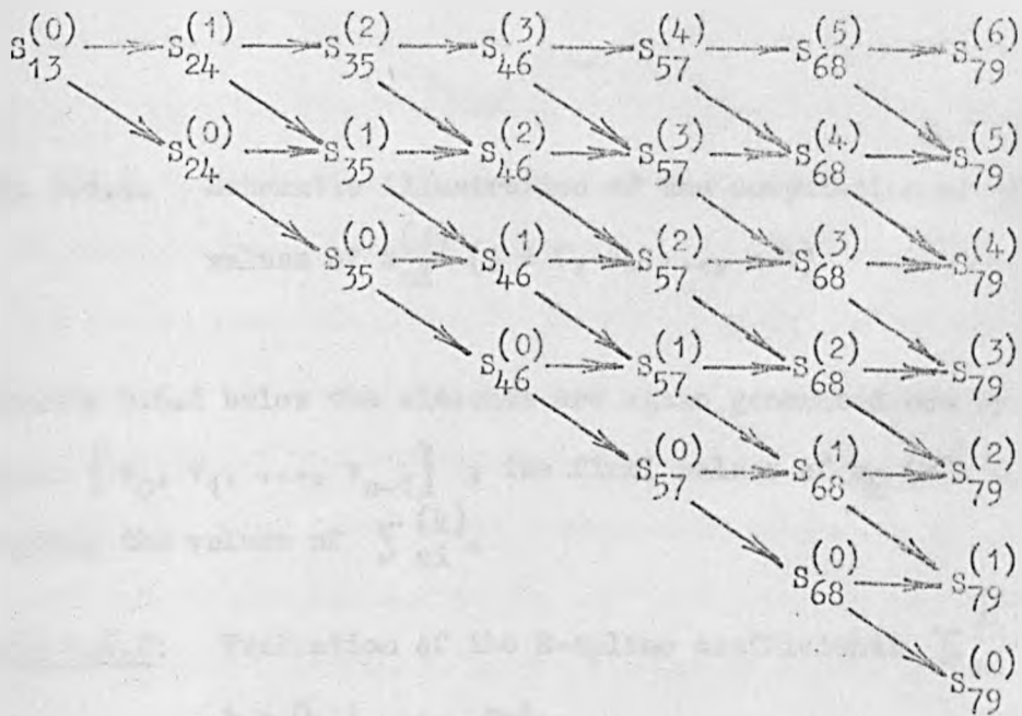
Fig 5.6.3. Schematic illustration of the computation of the values of \xi_{79}^{(j)} ( j = 0, 1, \dots, 6 ).
