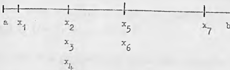
Fig. 3.1.1 A 3-extended partition
