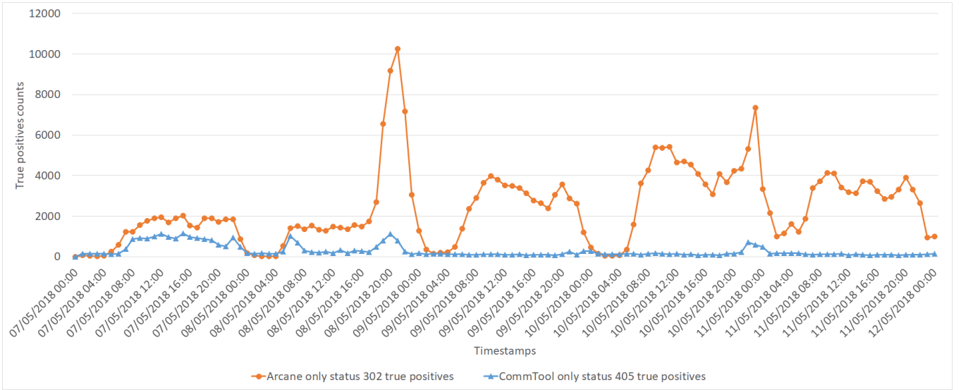
Fig. 5. Arcane only 302 and CommTool only 405 true positives.
