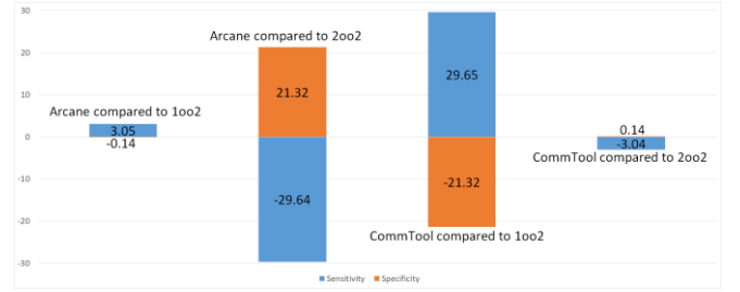
Fig. 1. Sensitivity and specificity changes from single tools to adjudication systems.
