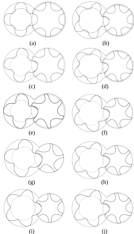
Fig. 3 Most popular screw compressor rotors today (a) Symmetric circular profile (Robert, 1952); (b) Lysholm's asymmetric profile (Lysholm, 1967); (c) SRM 'A' profile (Shibbye, 1979); (d) SKBK profile (Amosov, 1977); (e) SRM 'D' profile (Astberg, 1982); (f) Fusheng profile (Lee, 1988); (g) Compair profile (Hough et al. , 1984); (h) Hyper profile (Chen, 1995); (i) Rinder's profile (Rinder, 1987); (j) 'N' profile (Stosic, 1996)
