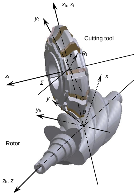
Fig. 12 Rotor and tool coordinate systems x_h, y_h, z_h rotor, x_t, y_t, z_t tool
