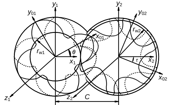
Fig. 7 Screw compressor rotors with parallel shafts and their coordinate systems
