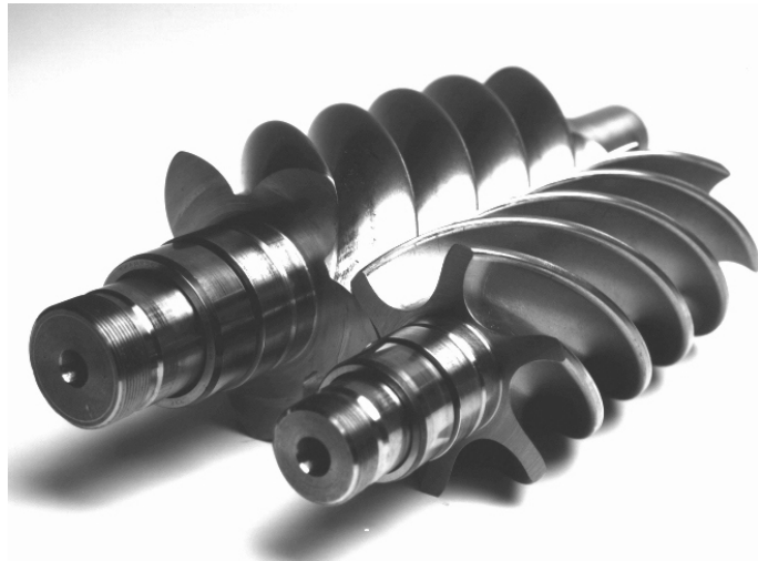
Figure 4 Drawing and photograph of 5/6 male and female 'N' rotors
