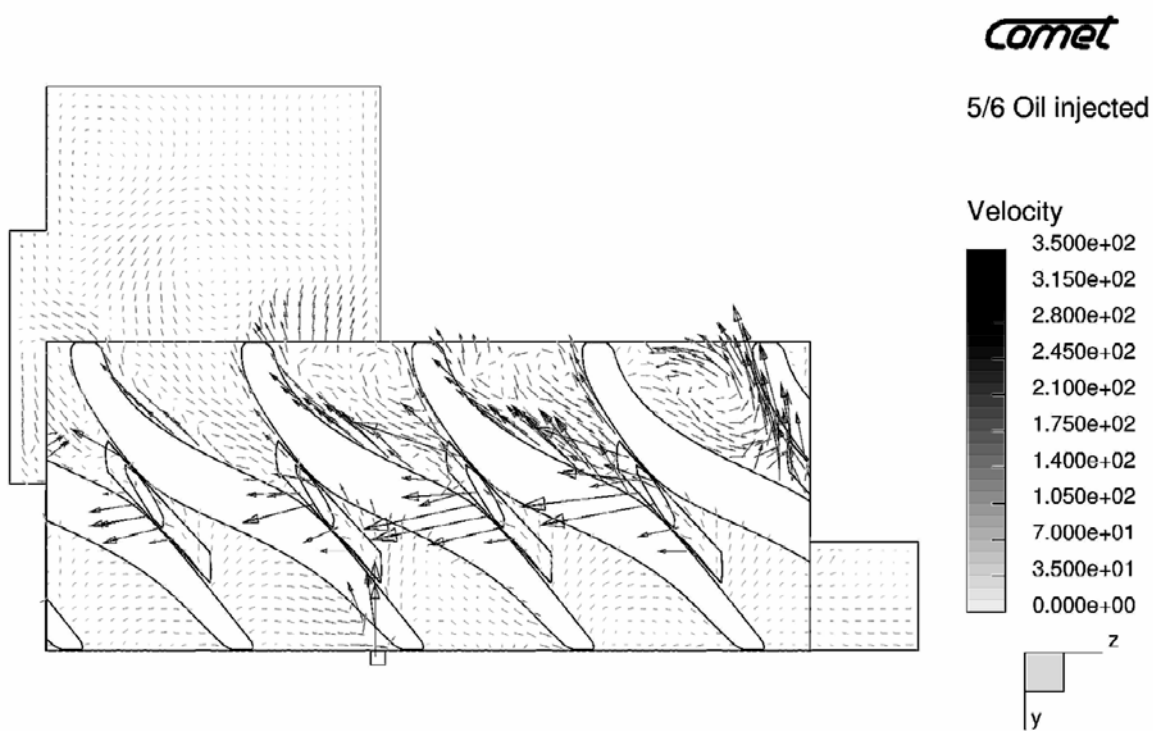
Figure 8 Velocity vectors in the compressor axial section
