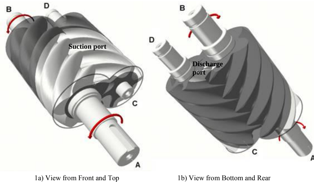
Fig. 1 Screw Compressor Main Components
