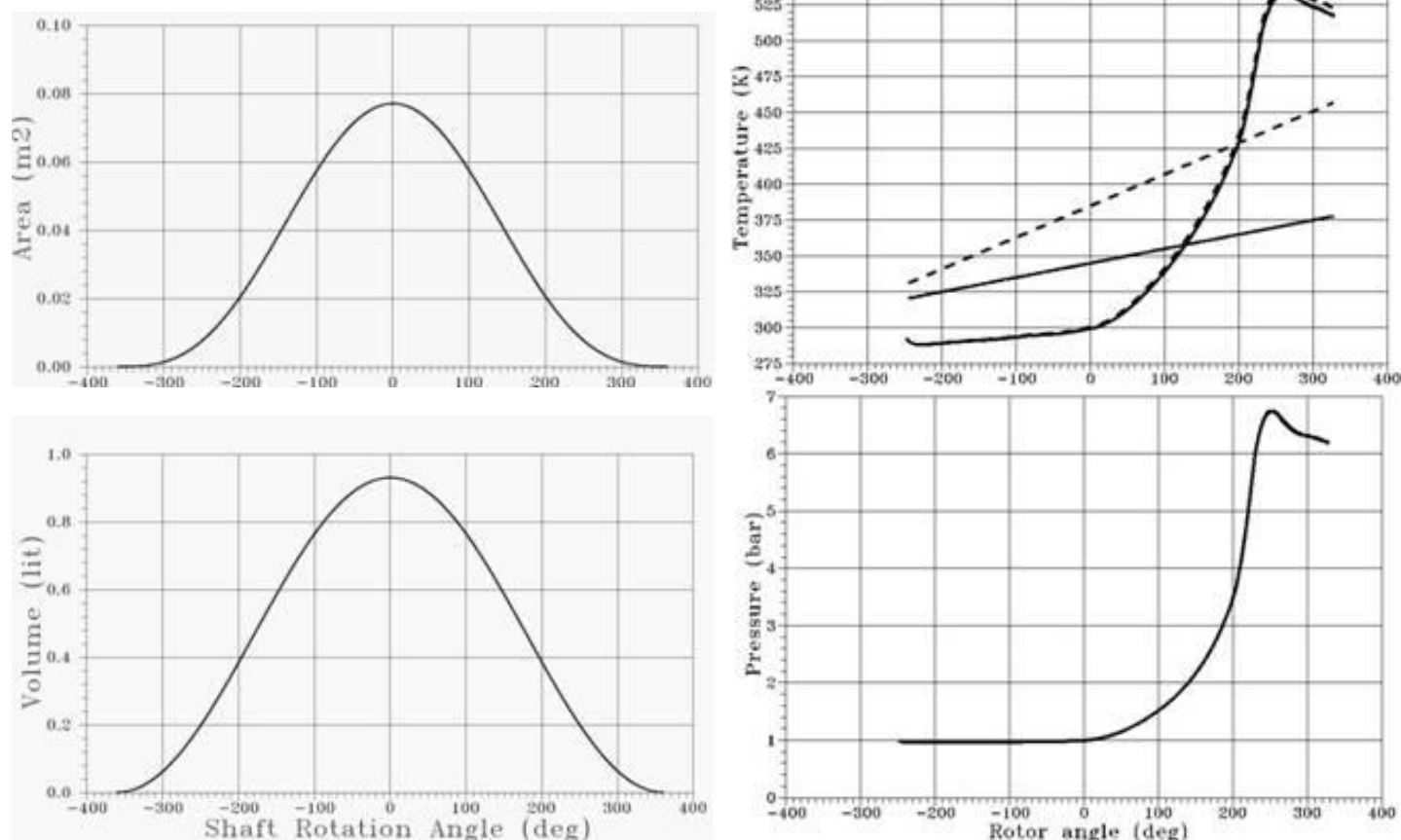
Fig. 3 Screw compressor heat transfer area, volume, temperature and pressure in function of shaft rotation angle
