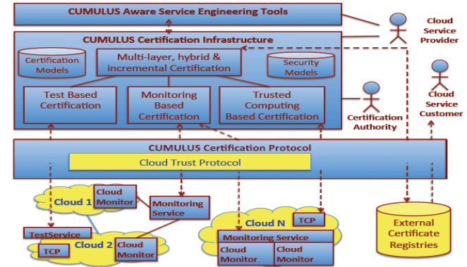
Figure 1: CUMULUS infrastructure
