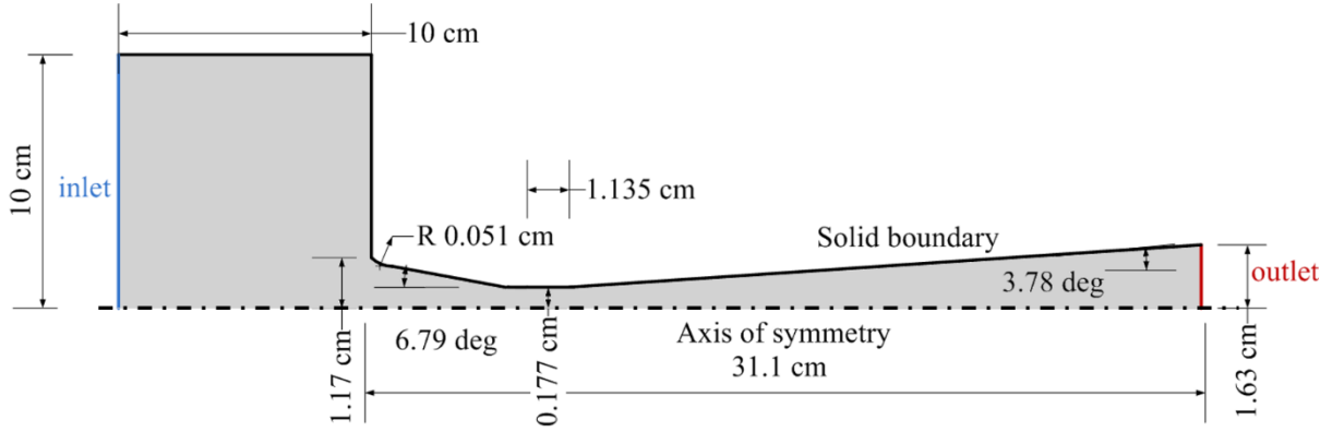
Figure 5: Geometry of the conical converging-diverging nozzle [12]. The inflow has been expanded upstream in order to impose the stagnation conditions of the experiment. The grey area denotes the computational domain, whereas inlet and outlet are coloured by blue and red respectively.
