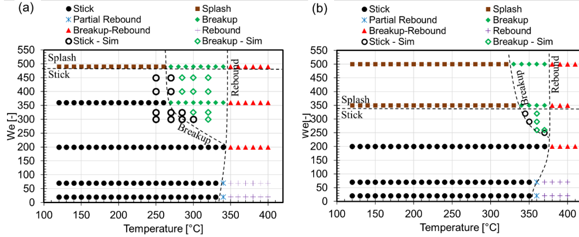
Figure 5: We-T regime diagram of Diesel fuel droplet impact on a heated aluminium surface at (a) P=1\text{bar} and (b) P=2\text{bar} . Empty markers show numerical results of the transition area of breakup regime have been added.
