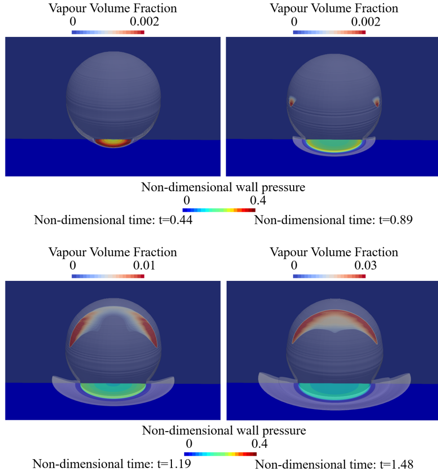
Figure 7: Drop impact at velocity 110 \text{ m/s} . Iso-surface of liquid mass fraction for Y_g = 0.5 combined with wall pressure (lower part) and vapour volume fraction (upper part). Pressure is divided by p_{wh} and time is measured from the moment of the impact and it has been non-dimensionalized with D/c_l .
