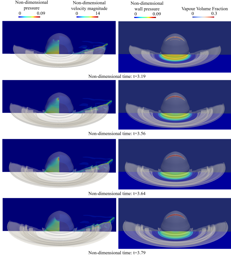
Figure 11: Later stage of drop impact at velocity 110 \text{ m/s} . Left figure: Iso-surface of liquid mass fraction for Y_g = 0.5 combined with pressure (left slice) and velocity magnitude (right slice). Right figure: Iso-surface of liquid mass fraction for Y_g = 0.5 combined with wall pressure (bottom slice) and vapour volume fraction (upper slice). Pressure and velocity are divided by p_{wh} and u_{imp} respectively, whereas time is measured from the moment of the impact and it has been non-dimensionalized with D/c_l .
