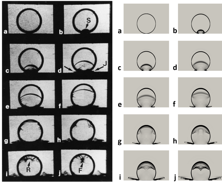
Figure 4: Validation of the numerical solution (right) against experiment (left) for a 2-D drop impact on a solid wall with impact velocity 110\text{ m/s} . The interframe time is t = 1\mu\text{s} . The left figure is taken from Field et. al [12].
