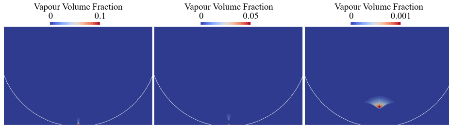
Figure 13: Close-up view of case 8 at non-dimensional times t = 0.15 (left), t = 0.18 (medium) and t = 0.25 (right). Slices of vapour volume fraction combined with iso-line of liquid mass fraction for Y_g = 0.5 are shown. Time has been non-dimensionalized with D/c_l .
