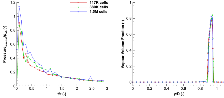
Figure 5: Grid independence study for three different grids (coarse, intermediate, fine). Maximum wall pressure with respect to time is shown on the left. The values of the vapour volume fraction on the right figure are exported at a line parallel to the y axis starting from x = 0.6 \text{ mm} , z = 0 at time T = 0.083 . Wall pressure is divided by p_{w,h} , time is measured from the moment of the impact and it is non-dimensionalized with \tau = D/c_l , whereas distance y has been divided by the drop diameter D .
