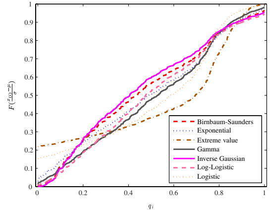
Fig. 5. The P-P plots for distributions Birnbaum-Saunders, Exponential, Extreme value, Gamma, Inverse Gaussian, Log-logistic, and Logistic.
