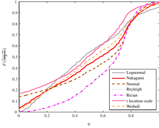
Fig. 6. The P-P plots for distributions Lognormal, Nakagami, Normal, Rayleigh, Rician, t-location scale, and Weibull.
