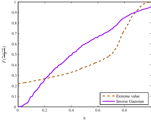
Fig. 7. The P-P plots for the Inverse Gaussian (i.e. the best fit) and the Extreme value (i.e. the worst fit).
