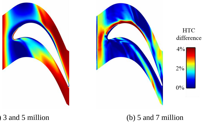
Figure 4.7: HTC difference distribution between the results from two meshes.
