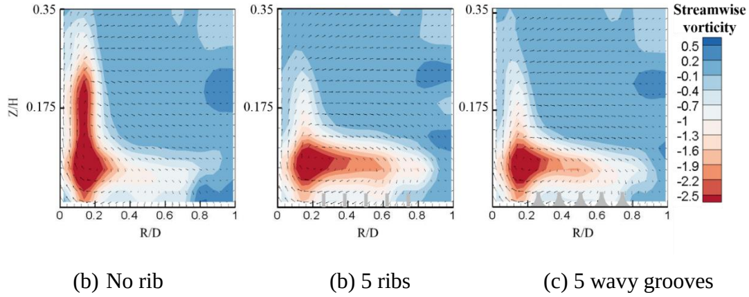
Figure 5.13: Dimensionless streamwise vorticity distributions obtained at 90-degree plane of the duct for cases (a) smooth (b) 5 ribs (c) 5 wavy grooves.
