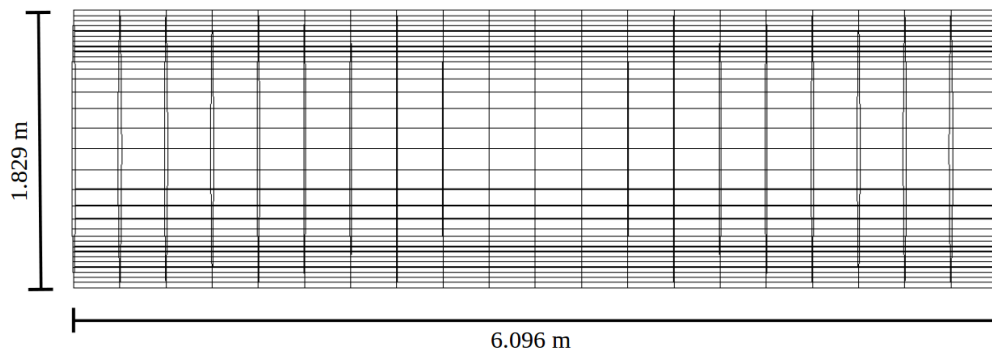
Figure 6.2: Goland Wing Surface Mesh
