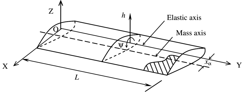
Figure 3.2: The coordinate system and notation for a bending-torsion coupled beam [81]
