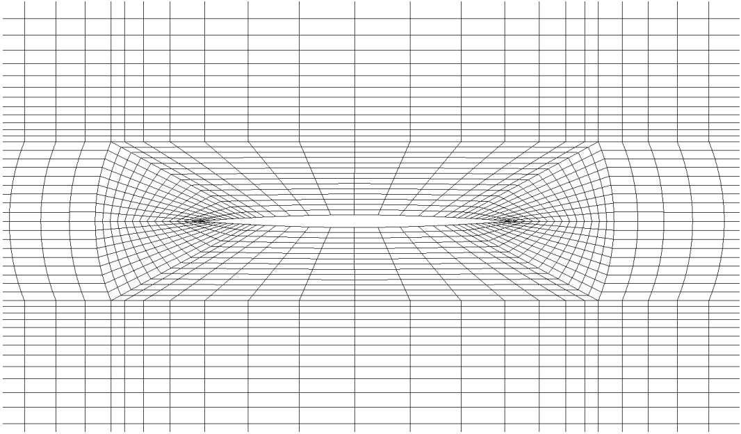
Figure 6.1: Mesh around Goland wing cross-section
