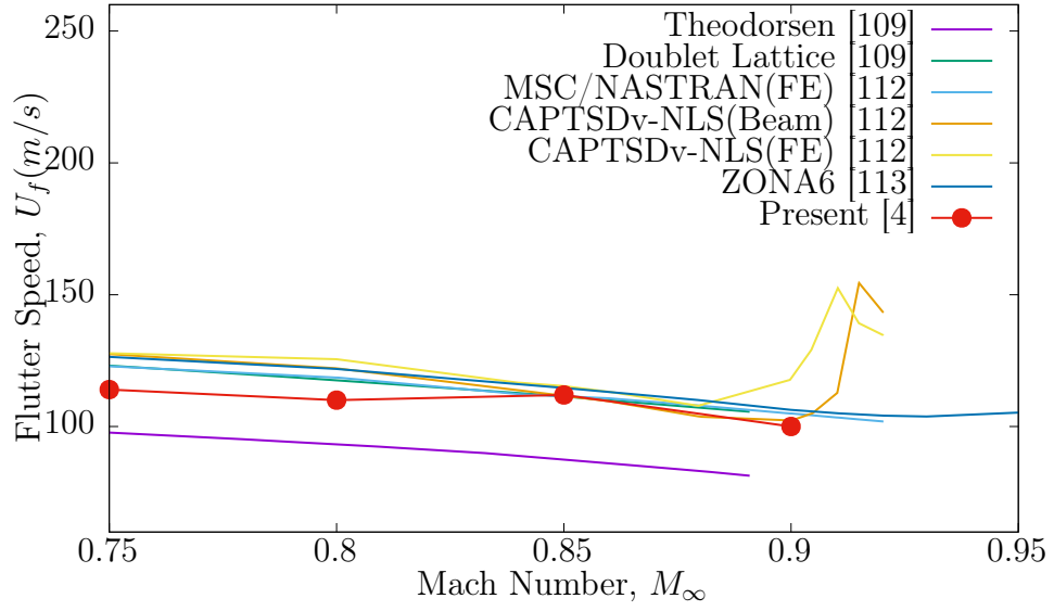
Figure 6.6: Flutter boundary for Goland Wing
