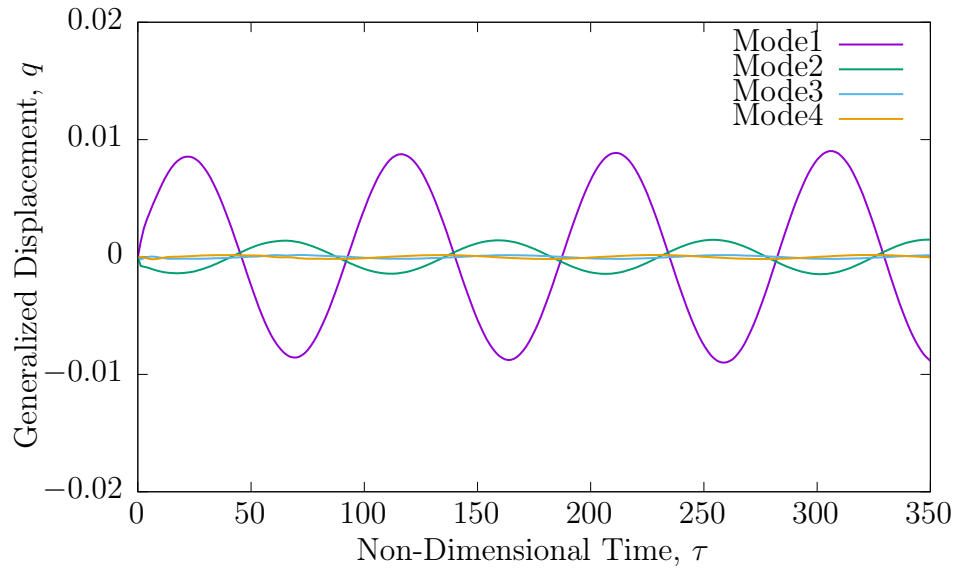
Figure 6.8: Near flutter point Response. M_\infty = 0.8 , V_\infty = 110 \text{ m/s}
