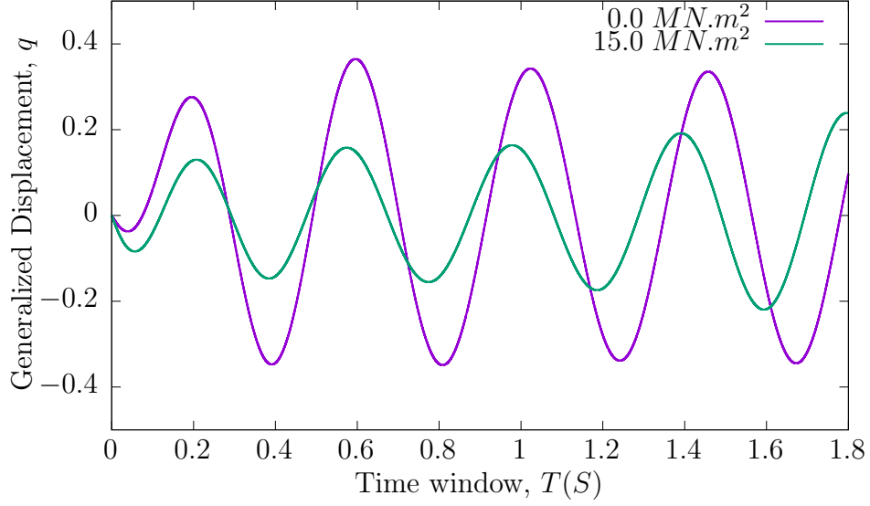
Figure 6.12: Near flutter point Response. M_\infty = 0.75 , V_\infty = 110m/s .
