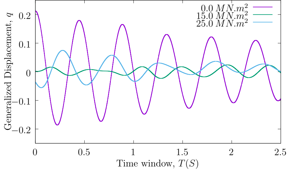
Figure 6.13: Near flutter point Response. M_\infty = 0.80 , V_\infty = 100 \text{ m/s} .
