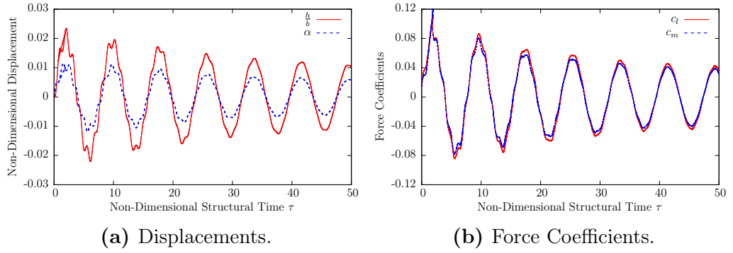
Figure 5.9: Damped Response. M_\infty = 0.85 , V^* = 0.439
