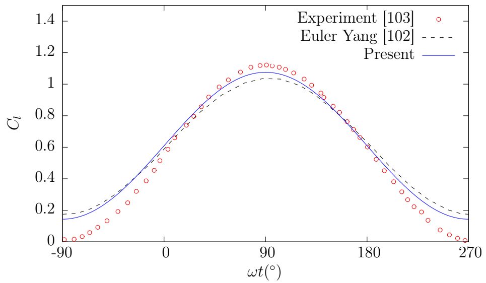
Figure 5.3: Instantaneous lift Coefficient
