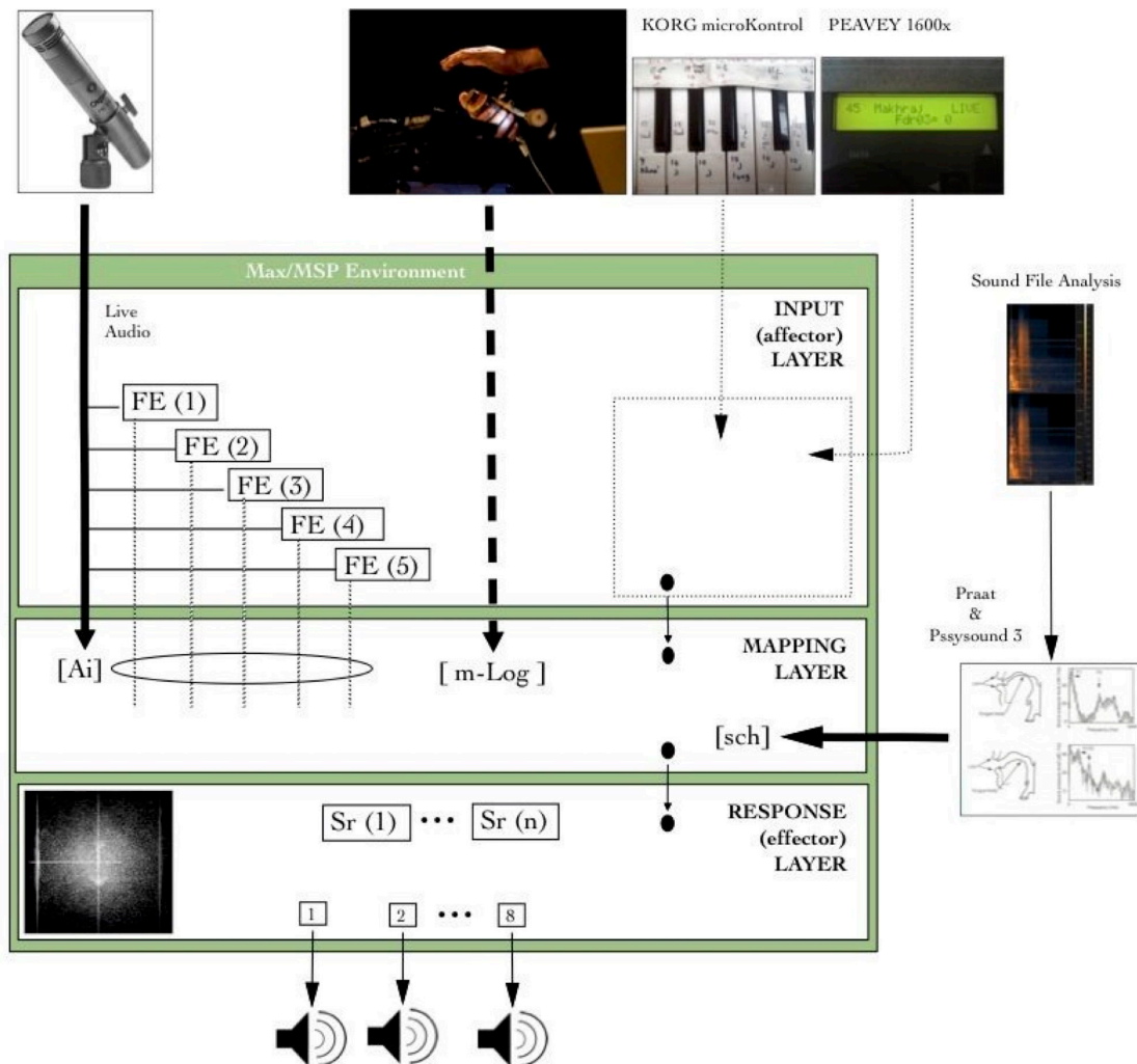
Figure 22: Schematic of signal flow in Makharej
