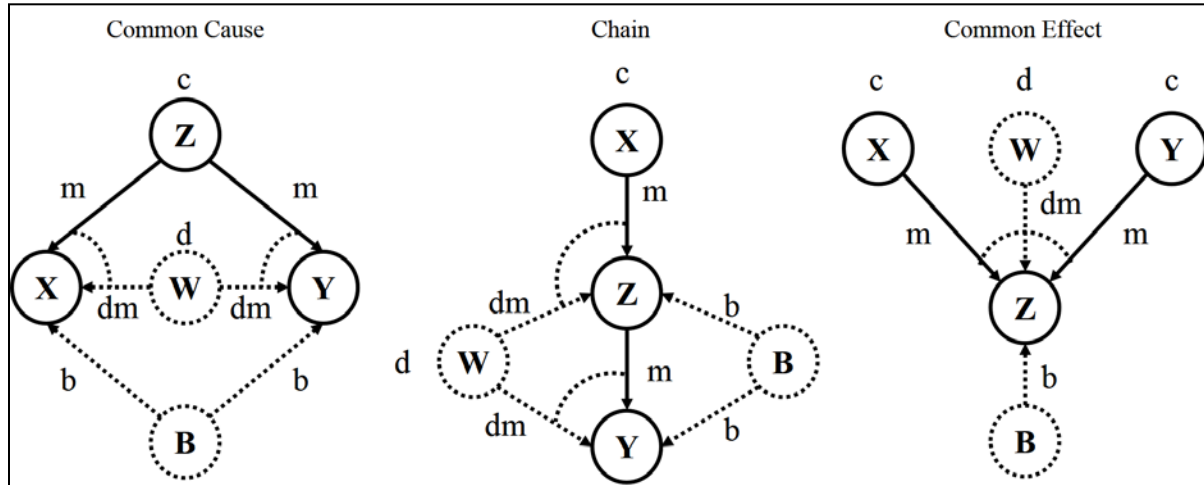
Fig. D5. Causal network structure defined by the specific shared disabler model (DISAB). The arrows show the direction of causality. Dotted lines and nodes represent variables that were not part of the experimental setup taught to participants but are auxiliary variables assumed by the model to be part of the participants' mental construction of the causal system (adapted from Rehder, 2014)
