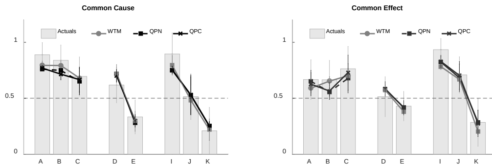
Fig. 10. Absolute judgments (dataset 2): Mean posterior predictive based on QPN, QPC, and WTM models compared to the mean actual behavior (gray bars).
