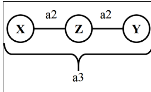
Fig. D4. Network structure defined by the Associative model (ASSC). The associative model does not assume any particular direction of causality (adapted from Rehder, 2014).
