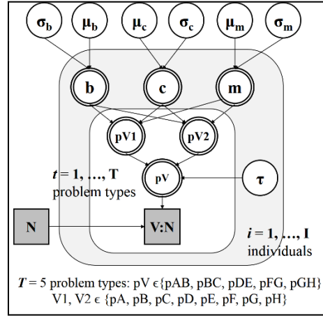
Fig. D2. Condensed graphical model for the normative causal graphical model [CGM]. The probabilities of states A to H are represented as pV1 and pV2 , repeated over the T = 5 different problem types. pV represents the respective relative probabilities \{pAB, pBC, pDE, pFG, pGH\} . The calculations for pV1_t and pV2_t can be represented simply as pV1_t = \text{CGM}(c_i, m_i, b_i, V1_t) and pV2_t = \text{CGM}(c_i, m_i, b_i, V2_t) , where \text{CGM}(c, m, b, V) is defined as per the detailed model. The notation V:N refers to the output of a binomial process with 2N trials, probability pV .
