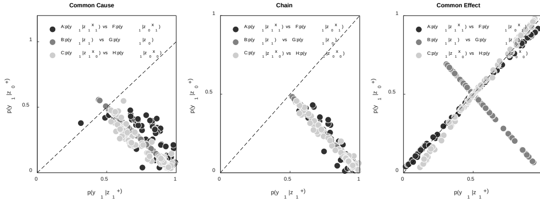
Fig. J1. Plausibility of intermediate absolute judgments (dataset 1): Comparison of intermediate absolute probability judgments generated by the clustered QPC model. Each dot represents the mean intermediate probability judgments for an individual. The x-axis plots the values when Z is present and the y-axis when Z is absent. The comparisons are made for comparable values of X (present, absent, unknown). Values to the right of the diagonal show judgments that are higher when Z is present compared to when Z is absent.
