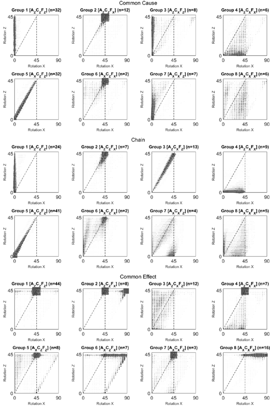
Fig. H1. Joint posterior probability density of the rotation parameters of the QPC model. The parameters are continuous but have been binned for this plot. The size of squares shows the value of the joint posterior probability density of the parameters within each cluster. Each cluster also shows the preferred projection orders for that cluster, and the number of participants for which this was the model cluster.
