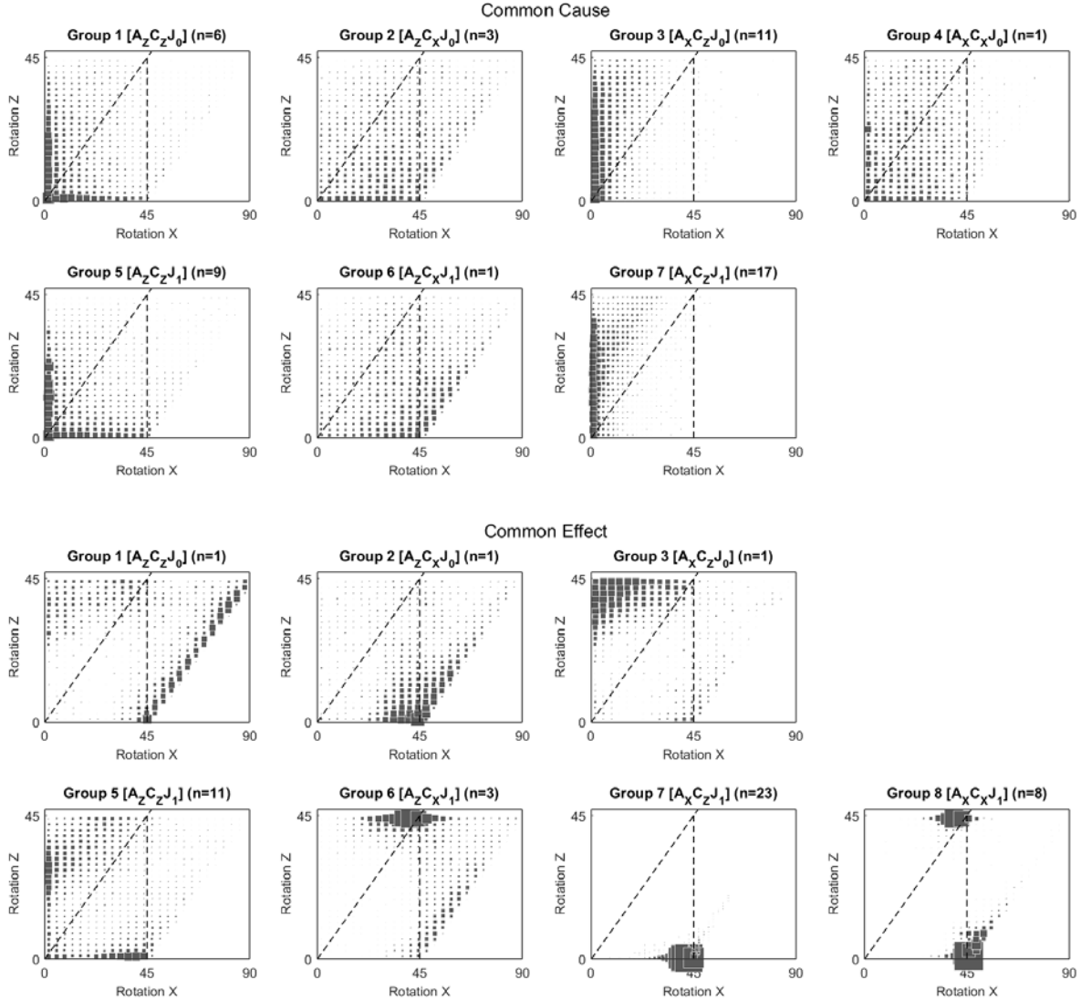
Fig. L1. Joint posterior probability density of the rotation parameters of the QPC model. The parameters are continuous but have been binned for this plot. The size of squares shows the value of the joint posterior probability density of the parameters within each cluster. Each cluster also shows the preferred projection orders for that cluster, and the number of participants for which this was the model cluster.
