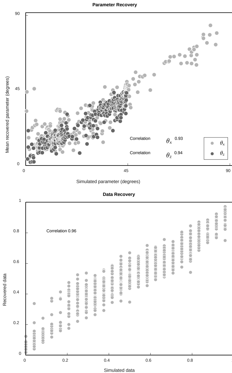
Fig. M1. Recovery of simulated rotation parameters and generated data by the QPC model
