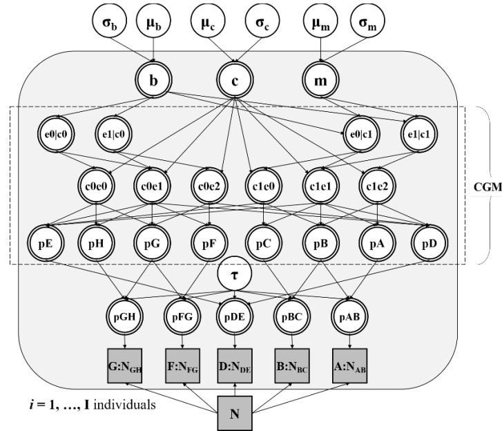
Fig. D3. Expanded graphical model for the normative causal graphical model [CGM]. Expanded graphical model for the CGM common cause network model (adapted from Rehder, 2014). In the figure, \{e0, e1, e2\} represent states with 0, 1 and 2 effects 'present', \{c0, c1\} represents states with the cause 'absent' and 'present' respectively. For example, (e1|c0) represents the independent probability of an effect being present conditional on the cause (Z) being absent, in this case being equal to b . Similarly, c0e1 represents the joint probability of a state with the primary cause absent and one of the two effects present. This can be derived as p(c0)p(e1|c0)p(e0|c0) , which is (1-c)b(1-b) . These joint probabilities can then be used to calculate the probability of each of the states A to H. For instance, state F represents a state with the primary cause being absent z0 , one effect being present x1 and the state of the second effect unknown. The probability of the second effect (Y) being present (denoted as pF ) can be calculated as pF =
