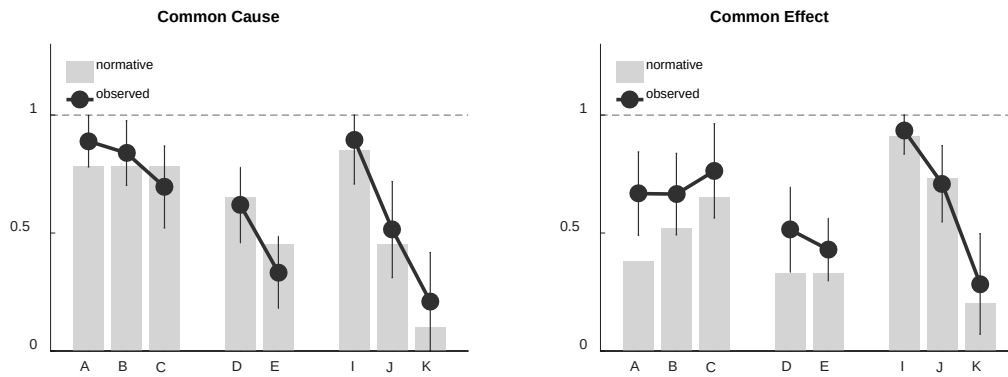
Fig. 3. Mean ratings for absolute judgments. The gray bars show the normative (rational) predictions derived from classical Bayes net principles, as reported in Rehder & Waldmann (2016). The line plots show the mean observed absolute probability judgments. The error bars represent a length of two standard deviations, centered on the mean (all adapted from Rehder & Waldmann, 2016).
