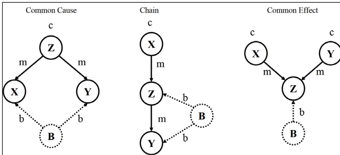
Fig. D1. Causal network structure defined by the normative causal graphical model (CGM). The arrows show the direction of causality. Dotted lines and nodes represent variables that were not part of the experimental setup taught to participants but are auxiliary variables assumed by the model to be part of the participants' mental construction of the causal system. (adapted from Rehder, 2014)
