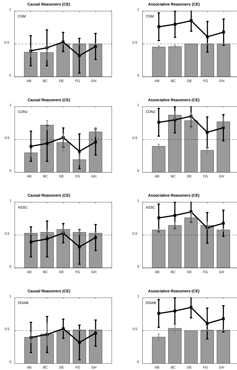
Fig. F3: Mean posterior predictive vs actuals by heuristic models (COMMON EFFECT)
