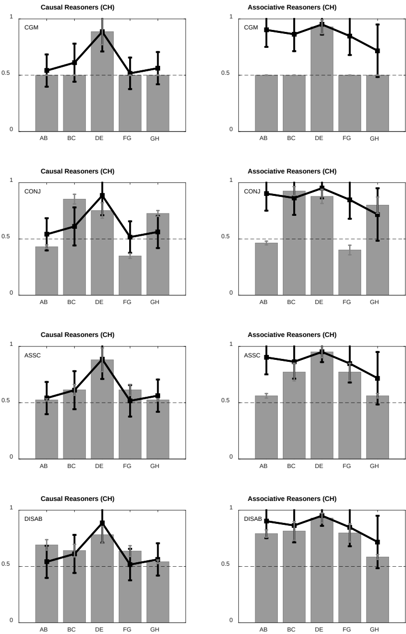
Fig. F2: Mean posterior predictive vs actuals by heuristic models (CHAIN)
