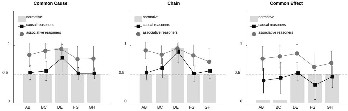
Fig. 2. Mean choice proportions for comparative judgments (AB represents the probability of selecting A vs B). The gray bars show the normative (rational) predictions derived from classical Bayes net principles including the causal Markov condition, and incorporating discounting into the inference for the common effect structure, as reported in Rehder (2014). The line plots show the actual observed aggregated choice responses for participants classified as causal and associative reasoners. The error bars represent a length of two standard deviations, centered on the mean (all adapted from Rehder, 2014).
