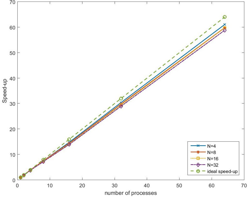
Figure 6: Speed-up for different number of monitoring dates N = 4, 8, 16, 32 . Ideal speed-up also included.
