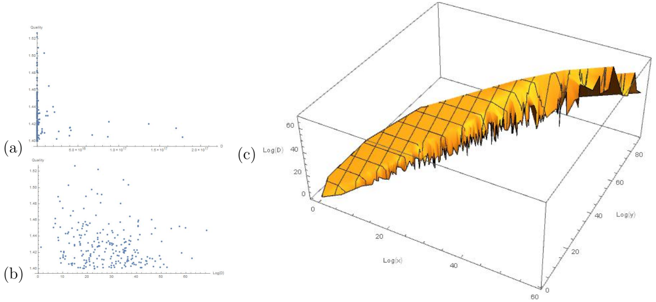
Figure 5: (a) A scatter plot of the D -parameter versus quality for the highest known quality examples of the ABC-triples; (b) The same as (a), but with log-axis for D ; (c) A 3D-scatter log-plot of the (x, y, D) values for these highest known quality cases.
