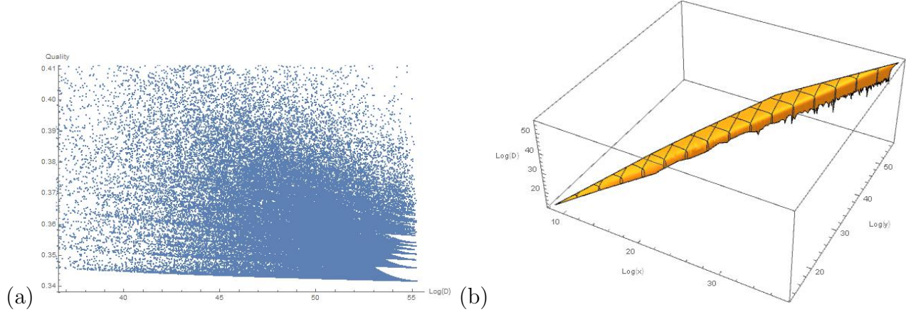
Figure 6: Sampling over 10^5 random ABC-triples, the corresponding points (x, y, D) on the curve E_D are found. (a) scatter plot for the the quality of the ABC-triple versus \log(D) ; (b) the log scatter plot of all (x, y, D) values.
