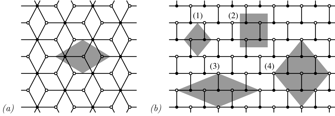
Figure 8: Dessins on the j = 0 or j = 54000 curves
