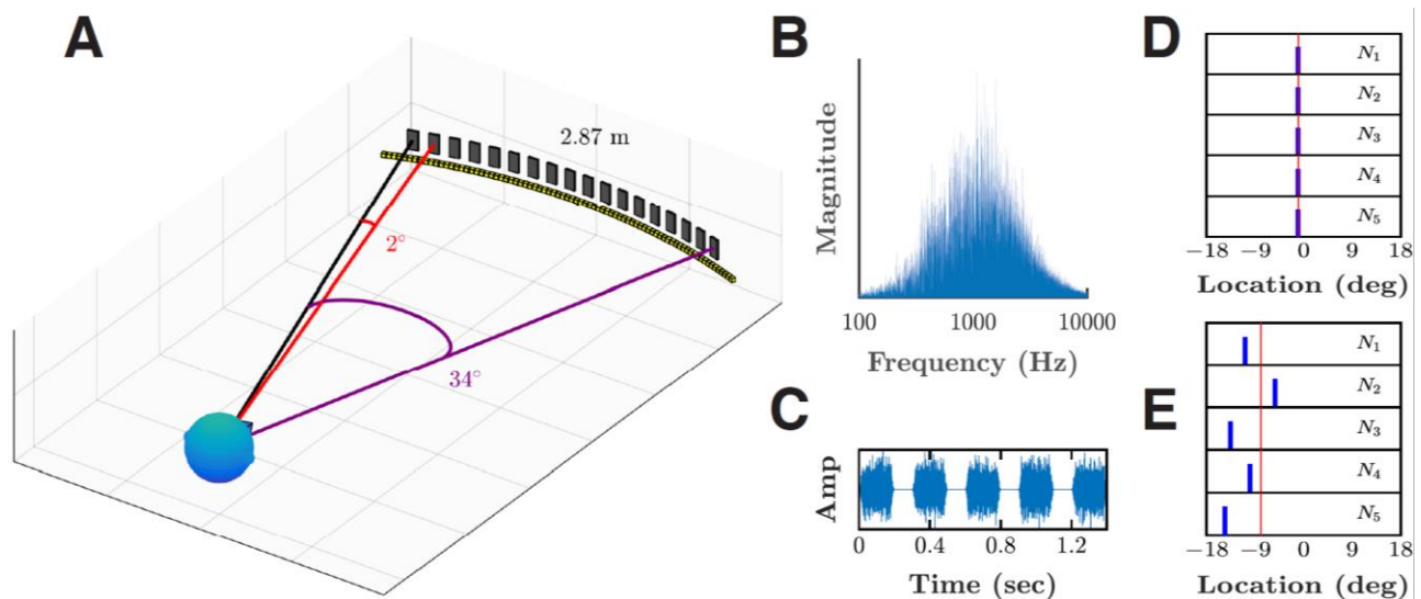
FIG 1. Stimuli and test apparatus for both experiments. (A) The listener's task was to locate the [single] source location of N noise bursts. Stimuli were presented along the azimuth, using 18 speakers distributed uniformly at 2^\circ intervals along a 34^\circ arc. Eighty LEDs arranged below the speakers were used for response-input, feedback, and fixation-cuing; (B) Each observation consisted of a 200 ms band-passed noise burst (1 octave bandwidth), centered at 1 kHz. (C) Each trial consisted of N observations (shown here: N = 5 ), presented sequentially with an inter-stimulus interval of 100 ms. (D) In Experiment I, N varied from 1 to 5, between blocks, in random order. Within each trial, the target location (thin red vertical line) varied randomly, and all sounds (thick blue lines) were presented at the target location (shown here: target = -1.25^\circ ). (E) In Experiment II, N was fixed at 5, and the location of each sound was randomly distributed around the target location, based on independent samples from a truncated-gaussian random variable (shown here: target = -9.25^\circ ).
