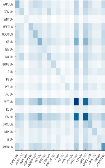
Graph A. Sample Covariance Matrix
