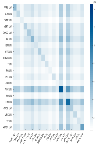
Graph B. Estimated Covariance Matrix
