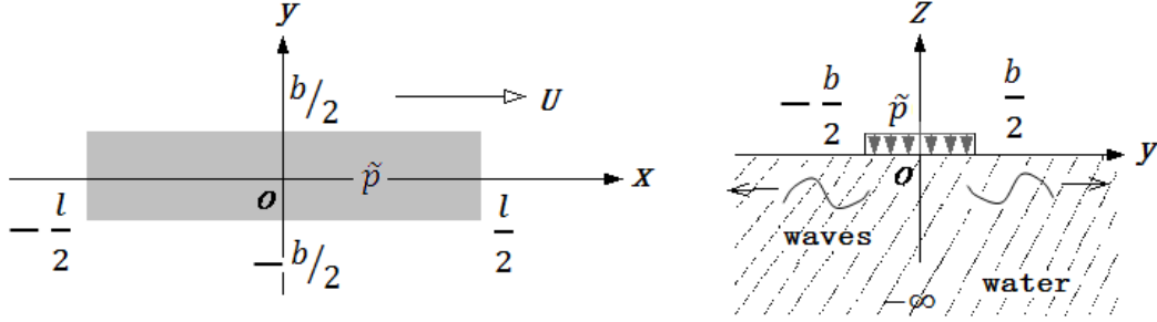
Fig. 4. Sketch of pulsating pressure without sidewalls (Left: top view; Right: front view).
