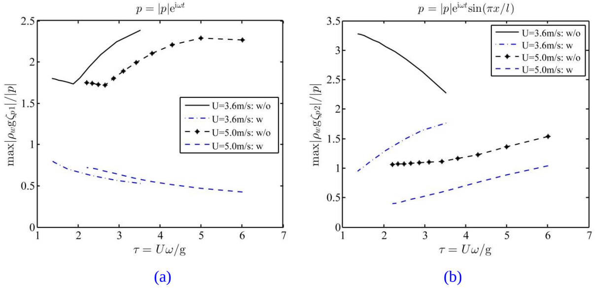
Fig. 8. Maximal amplitude of non-dimensional wave elevation at y = 0 due to the pulsating rectangular pressure patch: (a) p = |p|e^{i\omega t} ; (b) p = |p|e^{i\omega t} \sin \frac{\pi x}{l} . The legends 'w/o' means B = 0.24\text{m} while 'w' means B = 240\text{m} ( B is the breadth of pressure patch involved in Eq.(13)).
