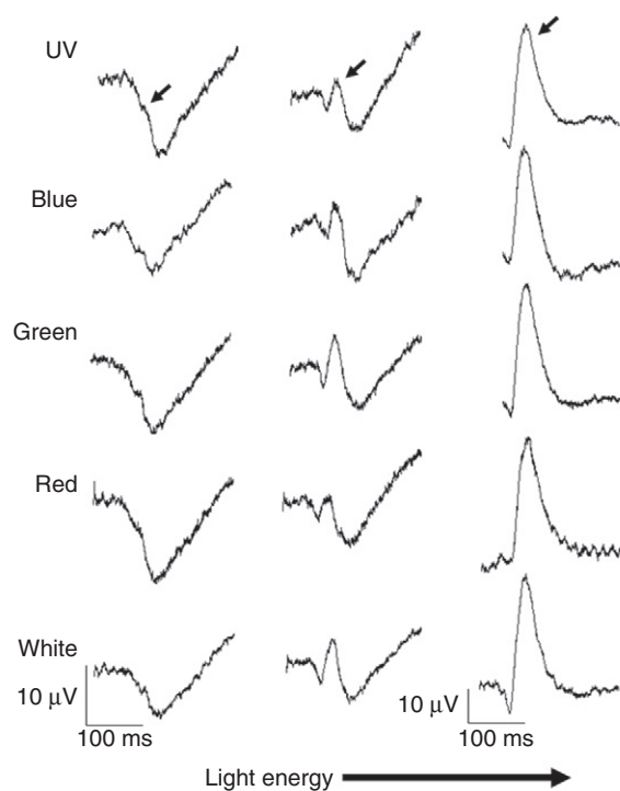
Fig. 2. Electrophoretogram (ERG) responses to increasing energy levels of UV, blue, green, red and white light stimulation in a representative reindeer. The b-wave (arrows) develops and increases in amplitude (positivity) with increasing energy. The intensity level required to generate a similar response using white light is approximately six times greater than that for the other stimuli. For each stimulus wavelength, the initial response is a marked negativity followed by an increasingly pronounced positivity (arrow). The response patterns were similar for each stimulus wavelength examined and this pattern was observed in the 18 reindeer tested. The responses shown for each stimulus is predominately within the mammalian rod range.
